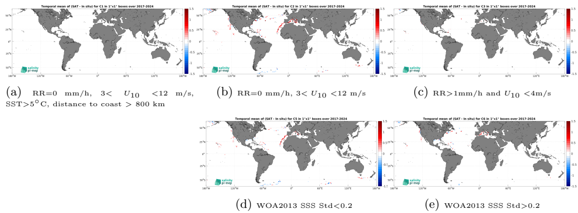
Figure 14: Temporal mean gridded over spatial boxes of size 1^\circ \times 1^\circ of \Delta SSS (SMOS SSS L4 OI v346 - Weekly (CMEMS-CATDS-LOPS) - Saildrone) for 5 different subdatasets corresponding to:RR=0 mm/h, 3 < U_{10} < 12 m/s, SST >5^\circ C, distance to coast > 800 km (a), RR=0 mm/h, 3 < U_{10} < 12 m/s (b), RR >1 mm/h and U_{10} < 4 m/s (c), WOA2013 SSS Std <0.2 (d), WOA2013 SSS Std >0.2 (e).
