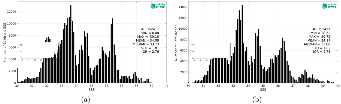
Figure 3: Histograms of SSS from Sailldrone (a) and SMOS SSS L4 OI v346 - Weekly (CMEMS-CATDS-LOPS) (b) considering all match-up pairs per bins of 0.1 over the SMOS coastal zone (<800km) 60N-60S Pi-MEP region and for the full satellite product period.
