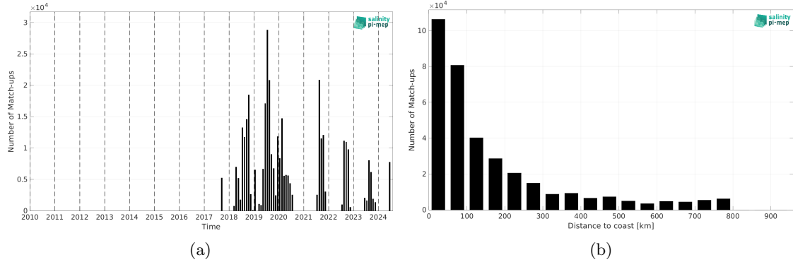
Figure 2: Number of match-ups between Sailldrone and SMOS SSS L4 OI v346 - Weekly (CMEMS-CATDS-LOPS) SSS as a function of time (a) and as function of the distance to coast (b) over the SMOS coastal zone (<800km) 60N-60S Pi-MEP region and for the full satellite product period.
