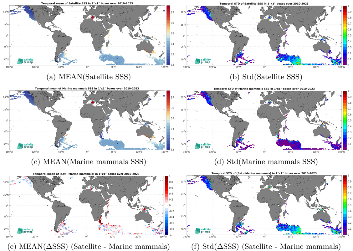
Figure 7: Temporal mean (left) and Std (right) of SSS from SMOS SSS L4 OI v346 - Weekly (CMEMS-CATDS-LOPS) (top), Marine mammals (middle), and of \Delta SSS (Satellite - Marine mammals). Only match-up pairs are used to generate these maps.
