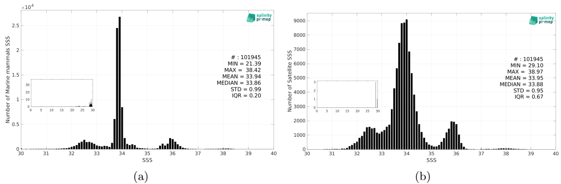
Figure 3: Histograms of SSS from Marine mammals (a) and SMOS SSS L4 OI v346 - Weekly (CMEMS-CATDS-LOPS) (b) considering all match-up pairs per bins of 0.1 over the SMOS coastal zone (<800km) 60N-60S Pi-MEP region and for the full satellite product period.
