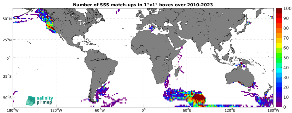
Figure 5: Number of SSS match-ups between Marine mammals SSS and the SMOS SSS L4 OI v346 - Weekly (CMEMS-CATDS-LOPS) SSS product for the SMOS coastal zone (<800km) 60N-60S Pi-MEP region over 1^\circ \times 1^\circ boxes and for the full satellite product period.
