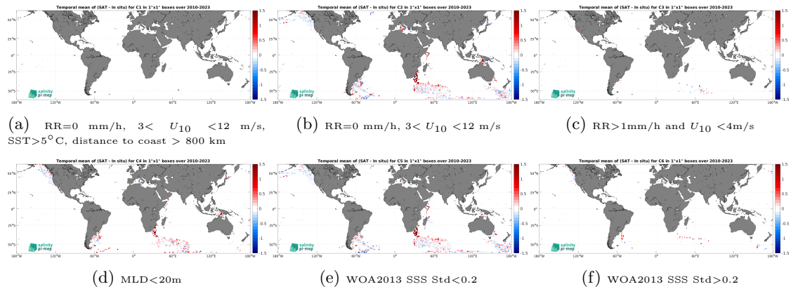
Figure 14: Temporal mean gridded over spatial boxes of size 1^\circ \times 1^\circ of \Delta SSS (SMOS SSS L4 OI v346 - Weekly (CMEMS-CATDS-LOPS) - Marine mammals) for 6 different subdatasets corresponding to:RR=0 mm/h, 3 < U_{10} < 12 m/s, SST>5°C, distance to coast > 800 km (a), RR=0 mm/h, 3 < U_{10} < 12 m/s (b), RR>1mm/h and U_{10} < 4 m/s (c),MLD<20m (d),WOA2013 SSS Std<0.2 (e),WOA2013 SSS Std>0.2 (f).
