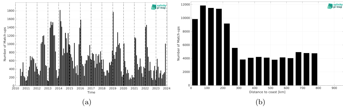
Figure 2: Number of match-ups between Marine mammals and SMOS SSS L4 OI v346 - Weekly (CMEMS-CATDS-LOPS) SSS as a function of time (a) and as function of the distance to coast (b) over the SMOS coastal zone (<800km) 60N-60S Pi-MEP region and for the full satellite product period.
