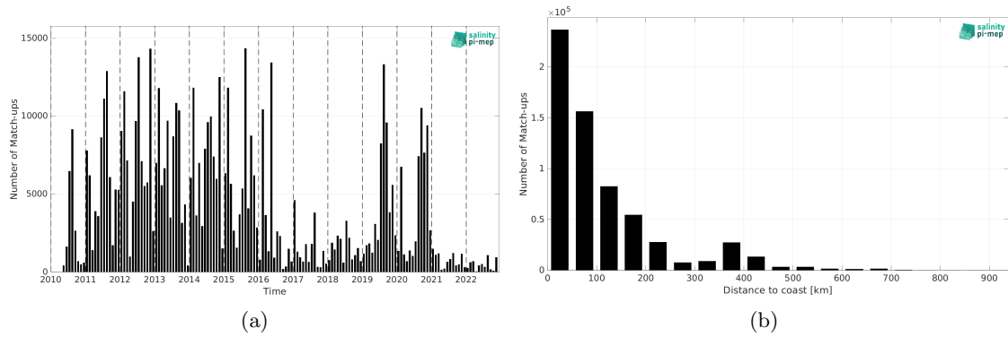
Figure 2: Number of match-ups between ICES and SMOS SSS L4 OI v346 - Weekly (CMEMS-CATDS-LOPS) SSS as a function of time (a) and as function of the distance to coast (b) over the SMOS coastal zone (<800km) 60N-60S Pi-MEP region and for the full satellite product period.
