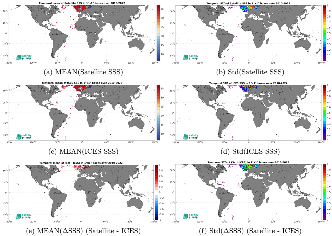
Figure 7: Temporal mean (left) and Std (right) of SSS from SMOS SSS L4 OI v346 - Weekly (CMEMS-CATDS-LOPS) (top), ICES (middle), and of \Delta SSS (Satellite - ICES). Only match-up pairs are used to generate these maps.
