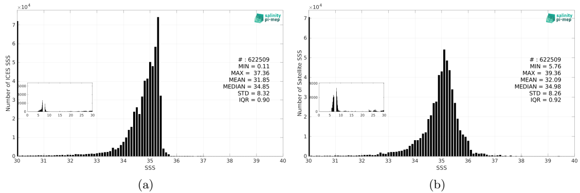
Figure 3: Histograms of SSS from ICES (a) and SMOS SSS L4 OI v346 - Weekly (CMEMS-CATDS-LOPS) (b) considering all match-up pairs per bins of 0.1 over the SMOS coastal zone (<800km) 60N-60S Pi-MEP region and for the full satellite product period.
