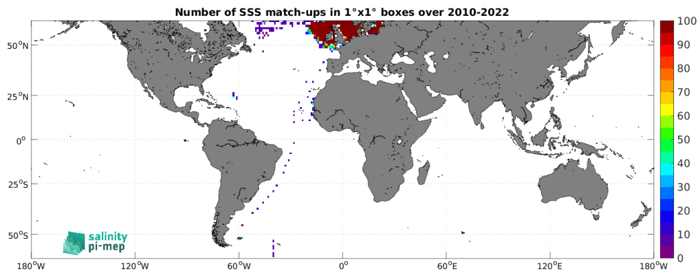
Figure 5: Number of SSS match-ups between ICES SSS and the SMOS SSS L4 OI v346 - Weekly (CMEMS-CATDS-LOPS) SSS product for the SMOS coastal zone (<800km) 60N-60S Pi-MEP region over 1^\circ \times 1^\circ boxes and for the full satellite product period.
