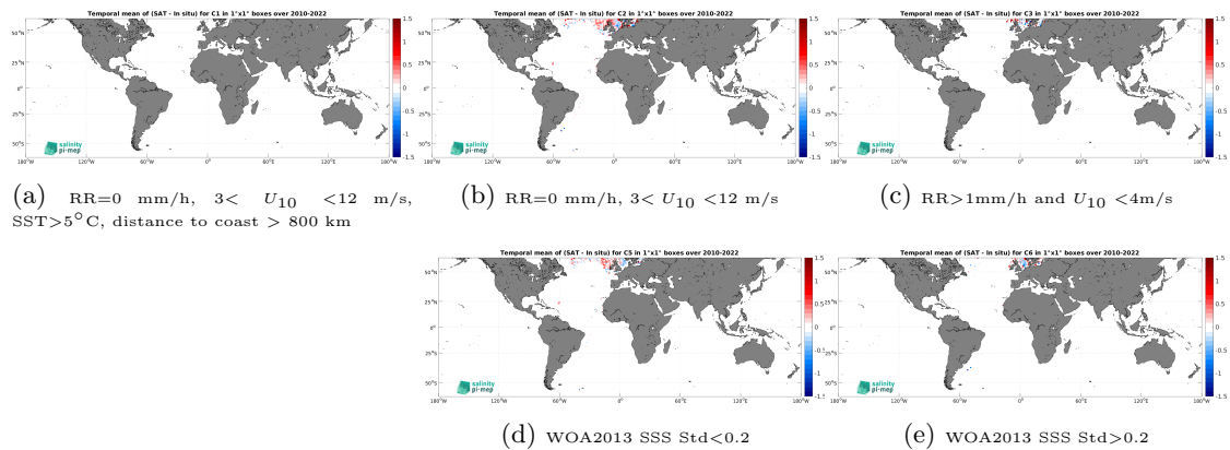
Figure 14: Temporal mean gridded over spatial boxes of size 1^\circ \times 1^\circ of \Delta SSS (SMOS SSS L4 OI v346 - Weekly (CMEMS-CATDS-LOPS) - ICES) for 5 different subdatasets corresponding to:RR=0 mm/h, 3 < U_{10} < 12 m/s, SST >5^\circ C, distance to coast > 800 km (a), RR=0 mm/h, 3 < U_{10} < 12 m/s (b), RR >1 mm/h and U_{10} < 4 m/s (c), WOA2013 SSS Std <0.2 (d), WOA2013 SSS Std >0.2 (e).
