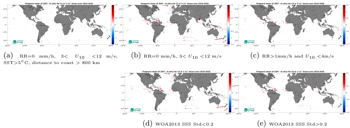
Figure 13: Temporal mean gridded over spatial boxes of size 1^\circ \times 1^\circ of \Delta\text{SSS} (SMOS SSS L4 OI v346 - Weekly (CMEMS-CATDS-LOPS) - Surface drifters) for 5 different subdatasets corresponding to:RR=0 mm/h, 3 < U_{10} < 12 m/s, SST >5^\circ\text{C} , distance to coast > 800 km (a), RR=0 mm/h, 3 < U_{10} < 12 m/s (b), RR >1 mm/h and U_{10} < 4 m/s (c), WOA2013 SSS Std <0.2 (d), WOA2013 SSS Std >0.2 (e).
