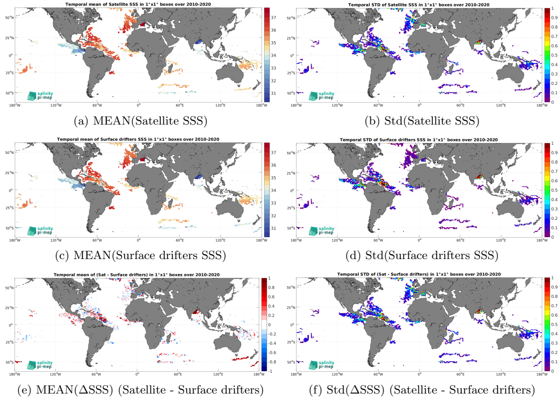
Figure 6: Temporal mean (left) and Std (right) of SSS from SMOS SSS L4 OI v346 - Weekly (CMEMS-CATDS-LOPS) (top), Surface drifters (middle), and of \Delta SSS (Satellite - Surface drifters). Only match-up pairs are used to generate these maps.
