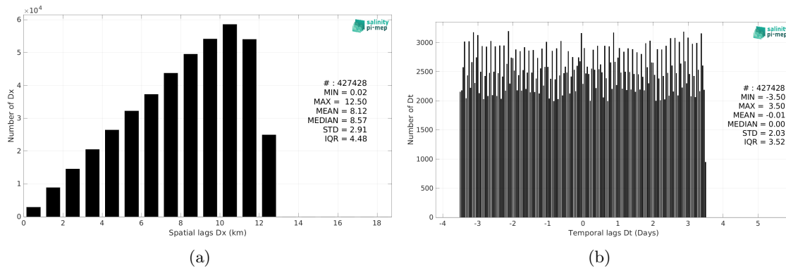
Figure 5: Histograms of the spatial (a) and temporal (b) lags between the location/time of the Surface drifters measurement and the date of the corresponding SMOS SSS L4 OI v346 - Weekly (CMEMS-CATDS-LOPS) SSS pixel.
