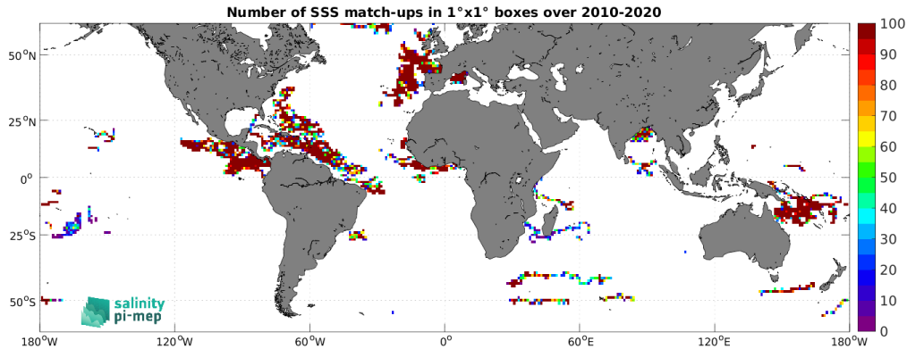
Figure 4: Number of SSS match-ups between Surface drifters SSS and the SMOS SSS L4 OI v346 - Weekly (CMEMS-CATDS-LOPS) SSS product for the SMOS coastal zone (<800km) 60N-60S Pi-MEP region over 1^\circ \times 1^\circ boxes and for the full satellite product period.
