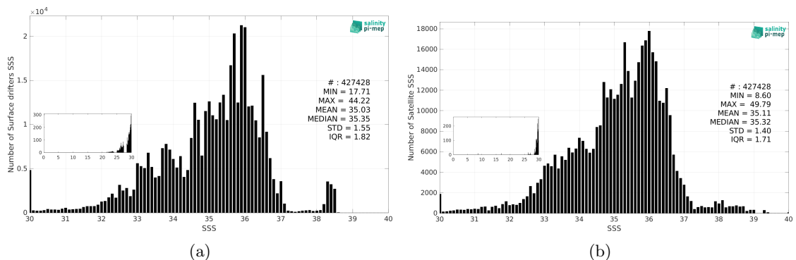
Figure 3: Histograms of SSS from Surface drifters (a) and SMOS SSS L4 OI v346 - Weekly (CMEMS-CATDS-LOPS) (b) considering all match-up pairs per bins of 0.1 over the SMOS coastal zone (<800km) 60N-60S Pi-MEP region and for the full satellite product period.
