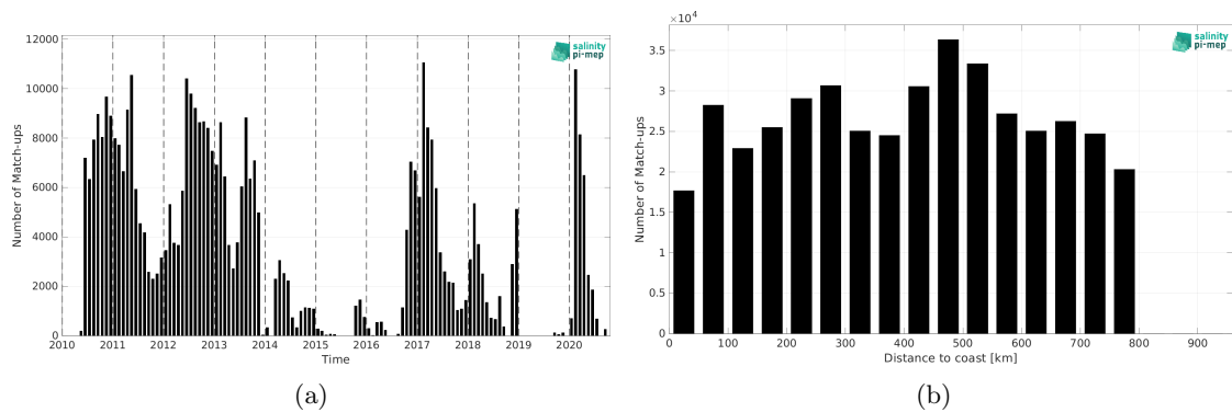
Figure 2: Number of match-ups between Surface drifters and SMOS SSS L4 OI v346 - Weekly (CMEMS-CATDS-LOPS) SSS as a function of time (a) and as function of the distance to coast (b) over the SMOS coastal zone (<800km) 60N-60S Pi-MEP region and for the full satellite product period.
