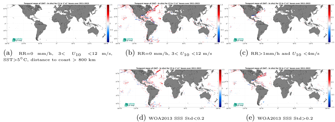
Figure 12: Temporal mean gridded over spatial boxes of size 1^\circ \times 1^\circ of \Delta SSS (SMOS SSS L4 OI v342 - Weekly (CMEMS-CATDS-LOPS) - TSG (SAMOS)) for 5 different subdatasets corresponding to:RR=0 mm/h, 3 < U_{10} < 12 m/s, SST >5^\circ C, distance to coast > 800 km (a), RR=0 mm/h, 3 < U_{10} < 12 m/s (b), RR >1 mm/h and U_{10} < 4 m/s (c), WOA2013 SSS Std <0.2 (d), WOA2013 SSS Std >0.2 (e).
