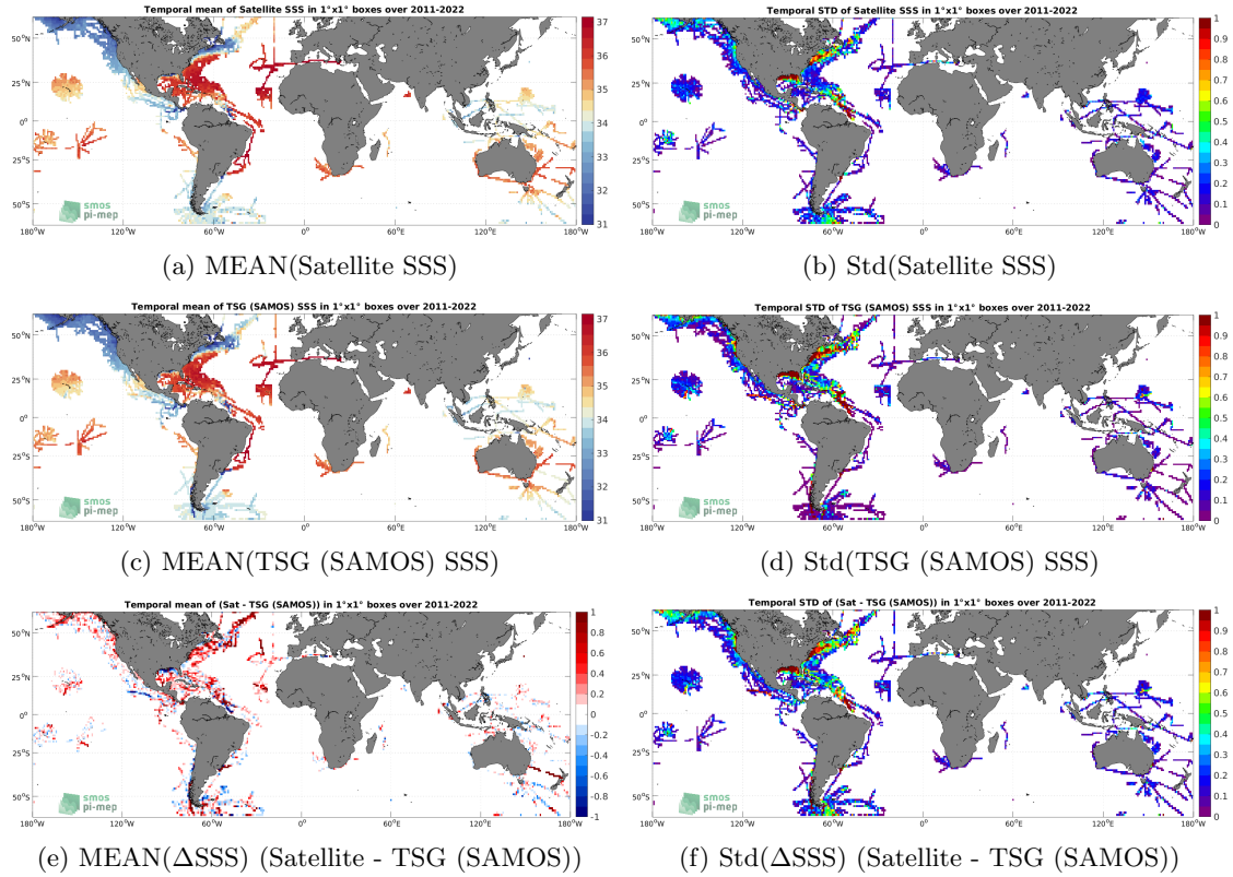
Figure 6: Temporal mean (left) and Std (right) of SSS from SMOS SSS L4 OI v342 - Weekly (CMEMS-CATDS-LOPS) (top), TSG (SAMOS) (middle), and of \Delta SSS (Satellite - TSG (SAMOS)). Only match-up pairs are used to generate these maps.
