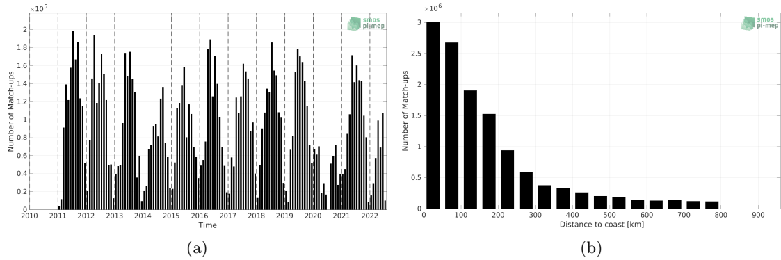
Figure 1: Number of match-ups between TSG (SAMOS) and SMOS SSS L4 OI v342 - Weekly (CMEMS-CATDS-LOPS) SSS as a function of time (a) and as function of the distance to coast (b) over the SMOS coastal zone (<800km) 60N-60S Pi-MEP region and for the full satellite product period.
