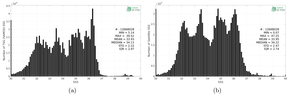
Figure 2: Histograms of SSS from TSG (SAMOS) (a) and SMOS SSS L4 OI v342 - Weekly (CMEMS-CATDS-LOPS) (b) considering all match-up pairs per bins of 0.1 over the SMOS coastal zone (<800km) 60N-60S Pi-MEP region and for the full satellite product period.
