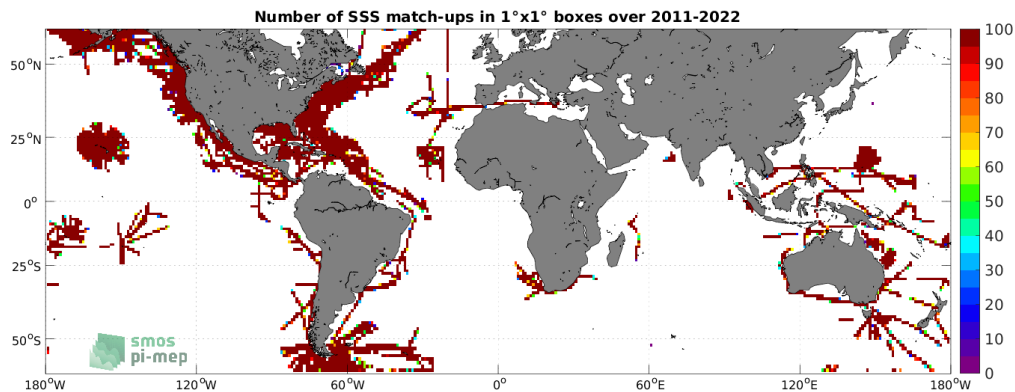
Figure 4: Number of SSS match-ups between TSG (SAMOS) SSS and the SMOS SSS L4 OI v342 - Weekly (CMEMS-CATDS-LOPS) SSS product for the SMOS coastal zone (<800km) 60N-60S Pi-MEP region over 1^\circ \times 1^\circ boxes and for the full satellite product period.
