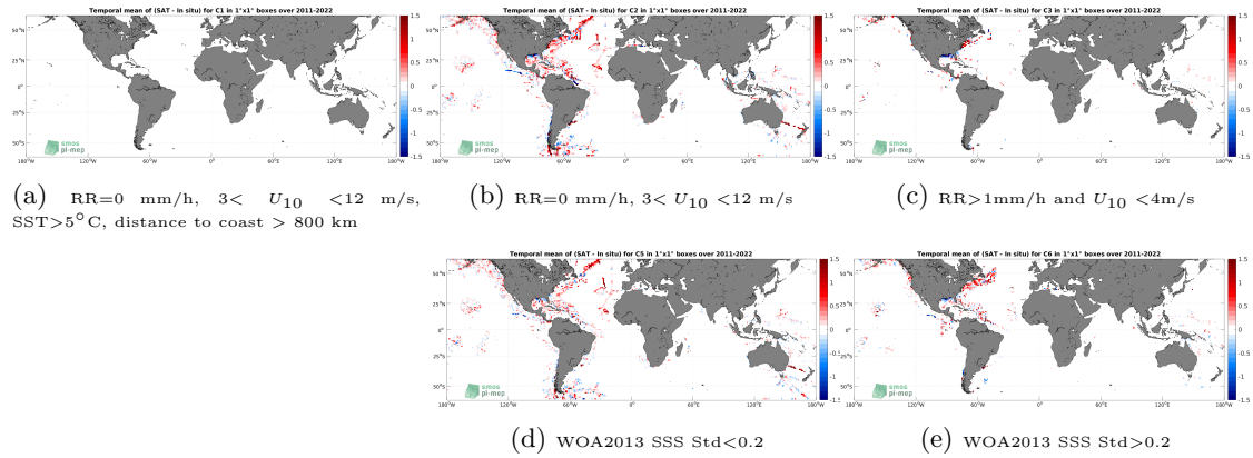
Figure 12: Temporal mean gridded over spatial boxes of size 1^\circ \times 1^\circ of \Delta\text{SSS} (SMOS SSS L4 OI v342 - Weekly (CMEMS-CATDS-LOPS) - TSG (SAMOS)) for 5 different subdatasets corresponding to:RR=0 mm/h, 3 < U_{10} < 12 m/s, SST >5^\circ\text{C} , distance to coast > 800 km (a), RR=0 mm/h, 3 < U_{10} < 12 m/s (b), RR >1 mm/h and U_{10} < 4 m/s (c), WOA2013 SSS Std <0.2 (d), WOA2013 SSS Std >0.2 (e).
