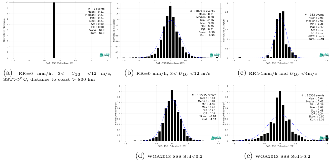
Figure 13: Normalized histogram of \Delta SSS (SMOS SSS L4 OI v342 - Weekly (CMEMS-CATDS-LOPS) - TSG (Polarstern)) for 5 different subdatasets corresponding to: RR=0 mm/h, 3 < U_{10} < 12 m/s, SST > 5°C, distance to coast > 800 km (a), RR=0 mm/h, 3 < U_{10} < 12 m/s (b), RR > 1mm/h and U_{10} < 4 m/s (c), WOA2013 SSS Std < 0.2 (d), WOA2013 SSS Std > 0.2 (e).
