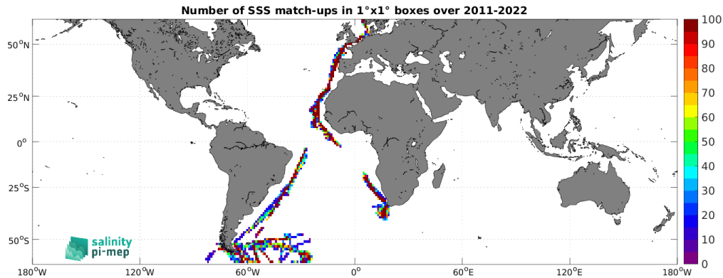
Figure 4: Number of SSS match-ups between TSG (Polarstern) SSS and the SMOS SSS L4 OI v342 - Weekly (CMEMS-CATDS-LOPS) SSS product for the SMOS coastal zone (<800km) 60N-60S Pi-MEP region over 1^\circ \times 1^\circ boxes and for the full satellite product period.
