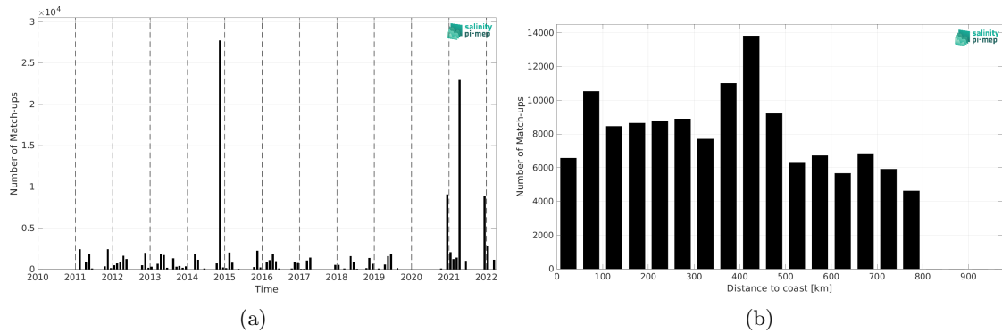
Figure 1: Number of match-ups between TSG (Polarstern) and SMOS SSS L4 OI v342 - Weekly (CMEMS-CATDS-LOPS) SSS as a function of time (a) and as function of the distance to coast (b) over the SMOS coastal zone (<800km) 60N-60S Pi-MEP region and for the full satellite product period.
