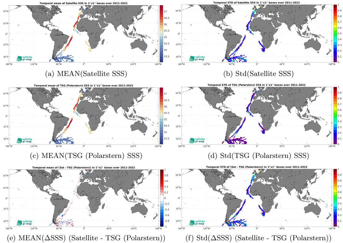
Figure 6: Temporal mean (left) and Std (right) of SSS from SMOS SSS L4 OI v342 - Weekly (CMEMS-CATDS-LOPS) (top), TSG (Polarstern) (middle), and of \Delta SSS (Satellite - TSG (Polarstern)). Only match-up pairs are used to generate these maps.
