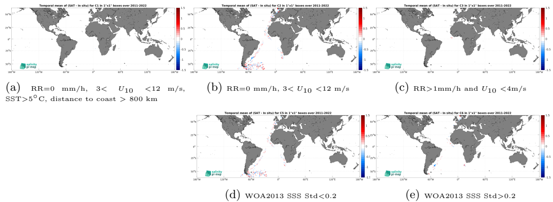
Figure 12: Temporal mean gridded over spatial boxes of size 1^\circ \times 1^\circ of \Delta SSS (SMOS SSS L4 OI v342 - Weekly (CMEMS-CATDS-LOPS) - TSG (Polarstern)) for 5 different subdatasets corresponding to:RR=0 mm/h, 3 < U_{10} < 12 m/s, SST >5^\circ\text{C} , distance to coast > 800 km (a), RR=0 mm/h, 3 < U_{10} < 12 m/s (b), RR >1 mm/h and U_{10} < 4 m/s (c), WOA2013 SSS Std <0.2 (d), WOA2013 SSS Std >0.2 (e).
