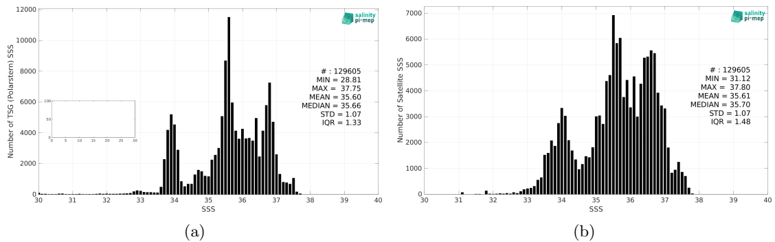
Figure 2: Histograms of SSS from TSG (Polarstern) (a) and SMOS SSS L4 OI v342 - Weekly (CMEMS-CATDS-LOPS) (b) considering all match-up pairs per bins of 0.1 over the SMOS coastal zone (<800km) 60N-60S Pi-MEP region and for the full satellite product period.
