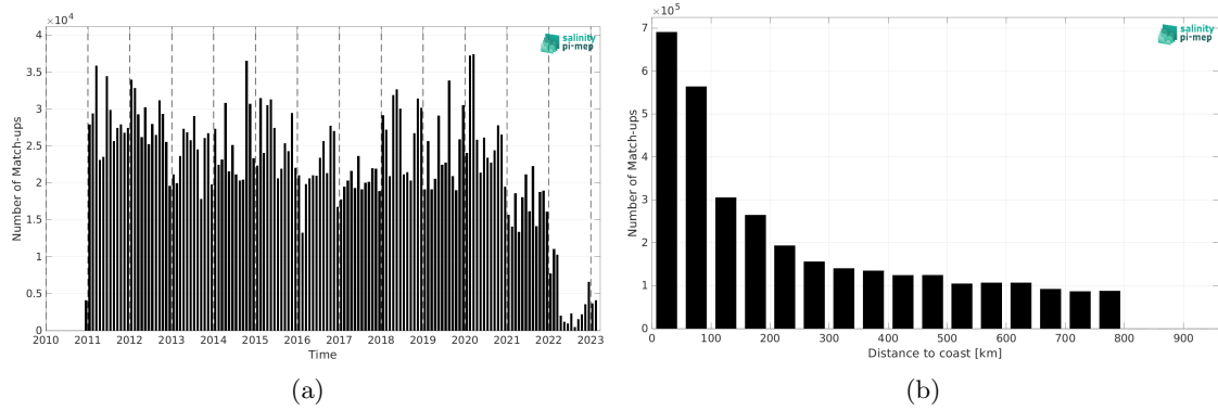
Figure 1: Number of match-ups between TSG (LEGOS-DM) and SMOS SSS L4 OI v342 - Weekly (CMEMS-CATDS-LOPS) SSS as a function of time (a) and as function of the distance to coast (b) over the SMOS coastal zone ( <800\text{km} ) 60N-60S Pi-MEP region and for the full satellite product period.
