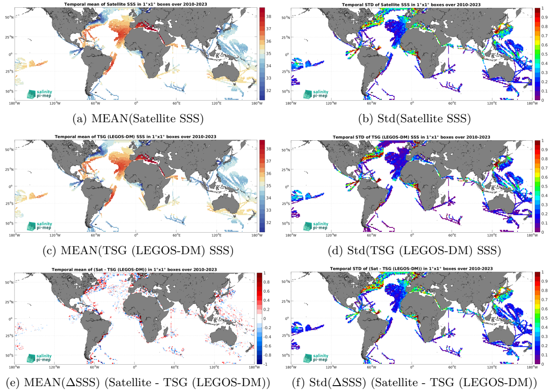
Figure 6: Temporal mean (left) and Std (right) of SSS from SMOS SSS L4 OI v342 - Weekly (CMEMS-CATDS-LOPS) (top), TSG (LEGOS-DM) (middle), and of \Delta SSS (Satellite - TSG (LEGOS-DM)). Only match-up pairs are used to generate these maps.
