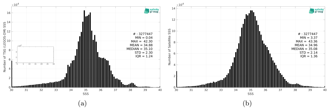
Figure 2: Histograms of SSS from TSG (LEGOS-DM) (a) and SMOS SSS L4 OI v342 - Weekly (CMEMS-CATDS-LOPS) (b) considering all match-up pairs per bins of 0.1 over the SMOS coastal zone ( <800\text{km} ) 60N-60S Pi-MEP region and for the full satellite product period.
