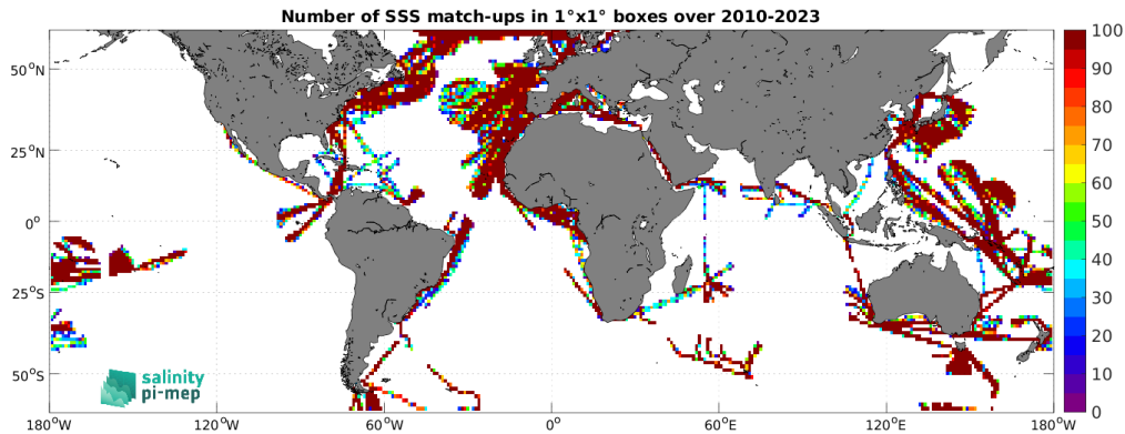
Figure 4: Number of SSS match-ups between TSG (LEGOS-DM) SSS and the SMOS SSS L4 OI v342 - Weekly (CMEMS-CATDS-LOPS) SSS product for the SMOS coastal zone (<800km) 60N-60S Pi-MEP region over 1^\circ \times 1^\circ boxes and for the full satellite product period.
