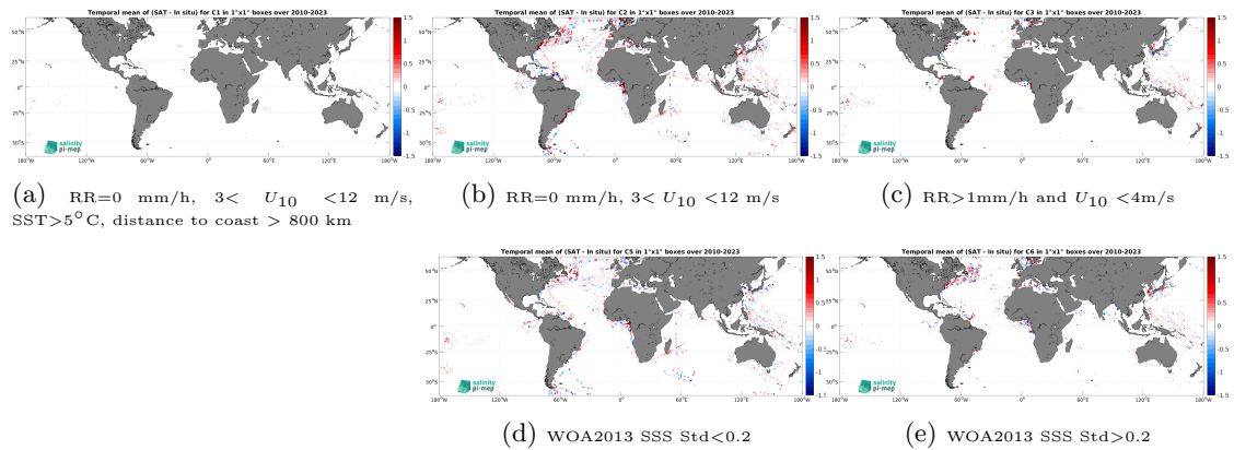
Figure 12: Temporal mean gridded over spatial boxes of size 1^\circ \times 1^\circ of \Delta\text{SSS} (SMOS SSS L4 OI v342 - Weekly (CMEMS-CATDS-LOPS) - TSG (LEGOS-DM)) for 5 different subdatasets corresponding to: RR=0 mm/h, 3 < U_{10} < 12 m/s, SST > 5^\circ\text{C} , distance to coast > 800 km (a), RR=0 mm/h, 3 < U_{10} < 12 m/s (b), RR > 1 mm/h and U_{10} < 4 m/s (c), WOA2013 SSS Std < 0.2 (d), WOA2013 SSS Std > 0.2 (e).
