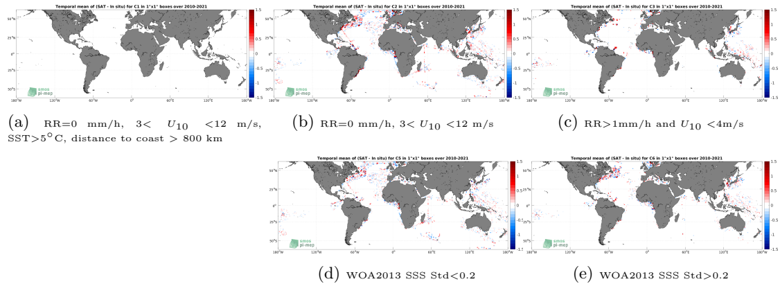
Figure 12: Temporal mean gridded over spatial boxes of size 1^\circ \times 1^\circ of \Delta SSS (SMOS SSS L4 OI v342 - Weekly (CMEMS-CATDS-LOPS) - TSG (LEGOS-DM)) for 5 different subdatasets corresponding to:RR=0 mm/h, 3 < U_{10} < 12 m/s, SST >5^\circ\text{C} , distance to coast > 800 km (a), RR=0 mm/h, 3 < U_{10} < 12 m/s (b), RR >1 mm/h and U_{10} < 4 m/s (c), WOA2013 SSS Std <0.2 (d), WOA2013 SSS Std >0.2 (e).
