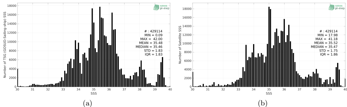
Figure 2: Histograms of SSS from TSG (GOSUD-Sailing-ship) (a) and SMOS SSS L4 OI v342 - Weekly (CMEMS-CATDS-LOPS) (b) considering all match-up pairs per bins of 0.1 over the SMOS coastal zone ( <800\text{km} ) 60N-60S Pi-MEP region and for the full satellite product period.
