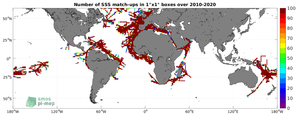
Figure 4: Number of SSS match-ups between TSG (GOSUD-Research-vessel) SSS and the SMOS SSS L4 OI v342 - Weekly (CMEMS-CATDS-LOPS) SSS product for the SMOS coastal zone (<800km) 60N-60S Pi-MEP region over 1^\circ \times 1^\circ boxes and for the full satellite product period.
