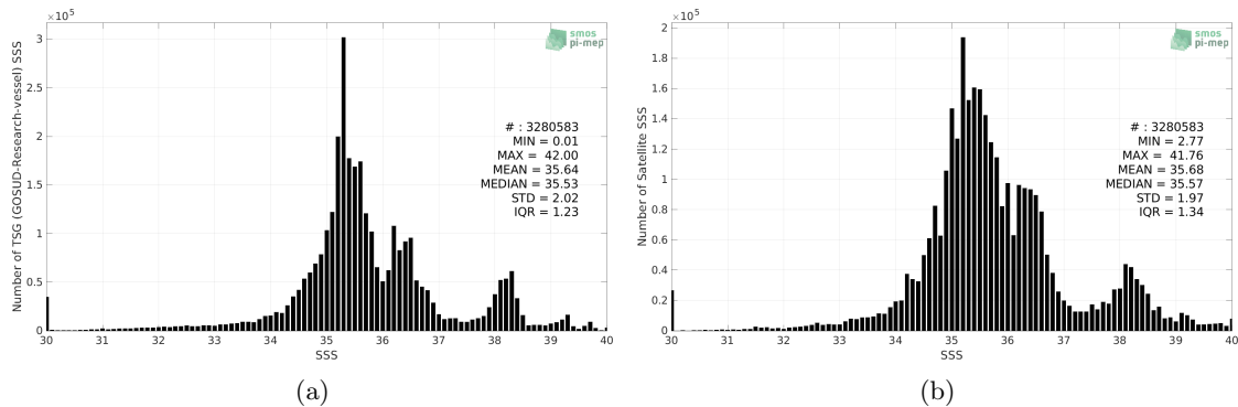
Figure 2: Histograms of SSS from TSG (GOSUD-Research-vessel) (a) and SMOS SSS L4 OI v342 - Weekly (CMEMS-CATDS-LOPS) (b) considering all match-up pairs per bins of 0.1 over the SMOS coastal zone (<800km) 60N-60S Pi-MEP region and for the full satellite product period.
