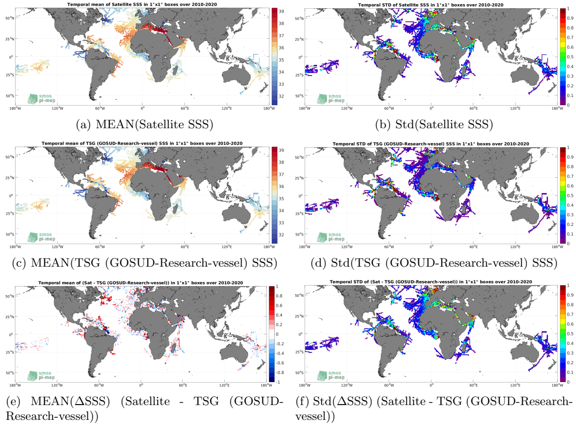
Figure 6: Temporal mean (left) and Std (right) of SSS from SMOS SSS L4 OI v342 - Weekly (CMEMS-CATDS-LOPS) (top), TSG (GOSUD-Research-vessel) (middle), and of \Delta SSS (Satellite - TSG (GOSUD-Research-vessel)). Only match-up pairs are used to generate these maps.
