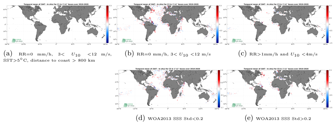
Figure 12: Temporal mean gridded over spatial boxes of size 1^\circ \times 1^\circ of \Delta SSS (SMOS SSS L4 OI v342 - Weekly (CMEMS-CATDS-LOPS) - TSG (GOSUD-Research-vessel)) for 5 different subdatasets corresponding to:RR=0 mm/h, 3 < U_{10} < 12 m/s, SST >5^\circ\text{C} , distance to coast > 800 km (a), RR=0 mm/h, 3 < U_{10} < 12 m/s (b), RR >1 mm/h and U_{10} < 4 m/s (c), WOA2013 SSS Std <0.2 (d), WOA2013 SSS Std >0.2 (e).
