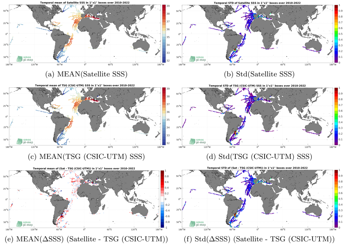
Figure 6: Temporal mean (left) and Std (right) of SSS from SMOS SSS L4 OI v342 - Weekly (CMEMS-CATDS-LOPS) (top), TSG (CSIC-UTM) (middle), and of \Delta SSS (Satellite - TSG (CSIC-UTM)). Only match-up pairs are used to generate these maps.
