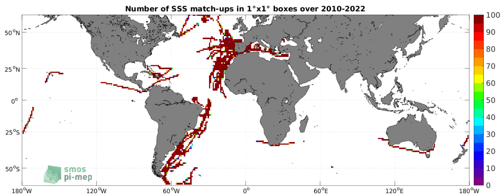
Figure 4: Number of SSS match-ups between TSG (CSIC-UTM) SSS and the SMOS SSS L4 OI v342 - Weekly (CMEMS-CATDS-LOPS) SSS product for the SMOS coastal zone (<800km) 60N-60S Pi-MEP region over 1^\circ \times 1^\circ boxes and for the full satellite product period.
