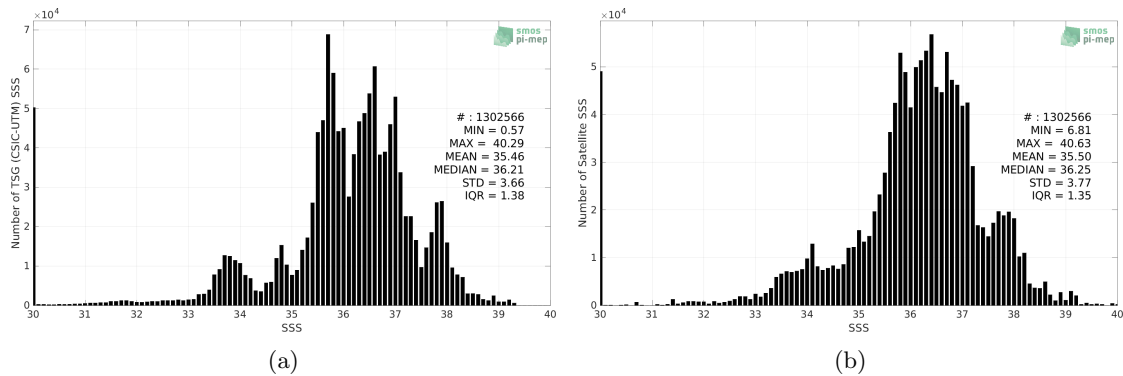
Figure 2: Histograms of SSS from TSG (CSIC-UTM) (a) and SMOS SSS L4 OI v342 - Weekly (CMEMS-CATDS-LOPS) (b) considering all match-up pairs per bins of 0.1 over the SMOS coastal zone (<800km) 60N-60S Pi-MEP region and for the full satellite product period.
