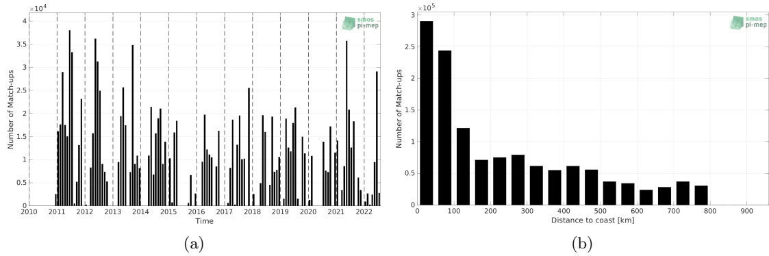
Figure 1: Number of match-ups between TSG (CSIC-UTM) and SMOS SSS L4 OI v342 - Weekly (CMEMS-CATDS-LOPS) SSS as a function of time (a) and as function of the distance to coast (b) over the SMOS coastal zone (<800km) 60N-60S Pi-MEP region and for the full satellite product period.
