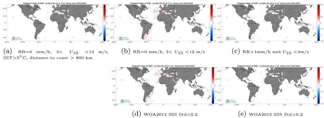
Figure 12: Temporal mean gridded over spatial boxes of size 1^\circ \times 1^\circ of \Delta SSS (SMOS SSS L4 OI v342 - Weekly (CMEMS-CATDS-LOPS) - TSG (CSIC-UTM)) for 5 different subdatasets corresponding to:RR=0 mm/h, 3 < U_{10} < 12 m/s, SST >5^\circ\text{C} , distance to coast > 800 km (a), RR=0 mm/h, 3 < U_{10} < 12 m/s (b), RR >1 mm/h and U_{10} < 4 m/s (c), WOA2013 SSS Std <0.2 (d), WOA2013 SSS Std >0.2 (e).
