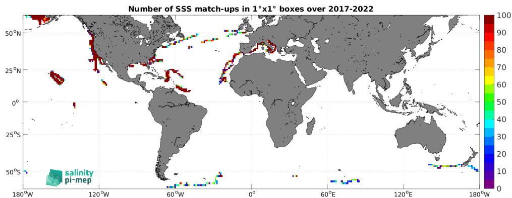
Figure 4: Number of SSS match-ups between Saildrone SSS and the SMOS SSS L4 OI v342 - Weekly (CMEMS-CATDS-LOPS) SSS product for the SMOS coastal zone (<800km) 60N-60S Pi-MEP region over 1^\circ \times 1^\circ boxes and for the full satellite product period.
