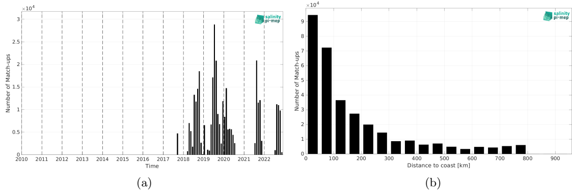
Figure 1: Number of match-ups between Saildrone and SMOS SSS L4 OI v342 - Weekly (CMEMS-CATDS-LOPS) SSS as a function of time (a) and as function of the distance to coast (b) over the SMOS coastal zone (<800km) 60N-60S Pi-MEP region and for the full satellite product period.
