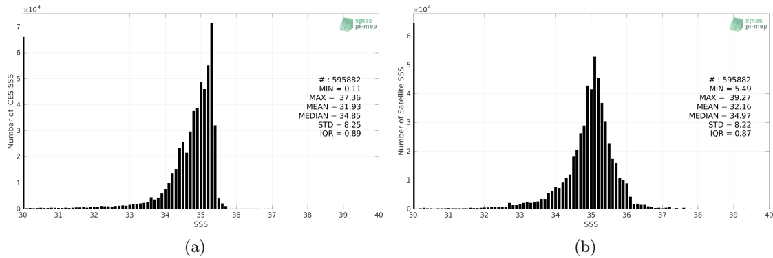
Figure 2: Histograms of SSS from ICES (a) and SMOS SSS L4 OI v342 - Weekly (CMEMS-CATDS-LOPS) (b) considering all match-up pairs per bins of 0.1 over the SMOS coastal zone (<800km) 60N-60S Pi-MEP region and for the full satellite product period.
