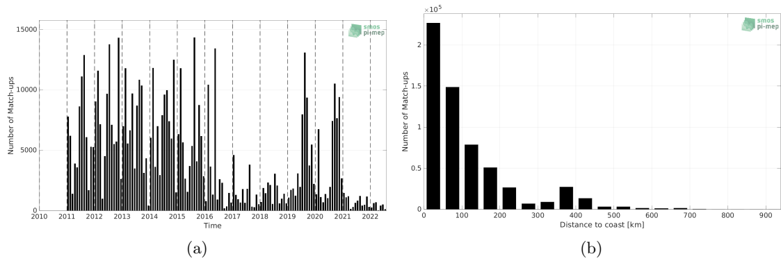
Figure 1: Number of match-ups between ICES and SMOS SSS L4 OI v342 - Weekly (CMEMS-CATDS-LOPS) SSS as a function of time (a) and as function of the distance to coast (b) over the SMOS coastal zone (<800km) 60N-60S Pi-MEP region and for the full satellite product period.
