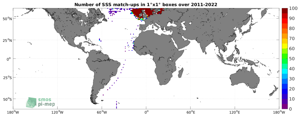
Figure 4: Number of SSS match-ups between ICES SSS and the SMOS SSS L4 OI v342 - Weekly (CMEMS-CATDS-LOPS) SSS product for the SMOS coastal zone (<800km) 60N-60S Pi-MEP region over 1^\circ \times 1^\circ boxes and for the full satellite product period.
