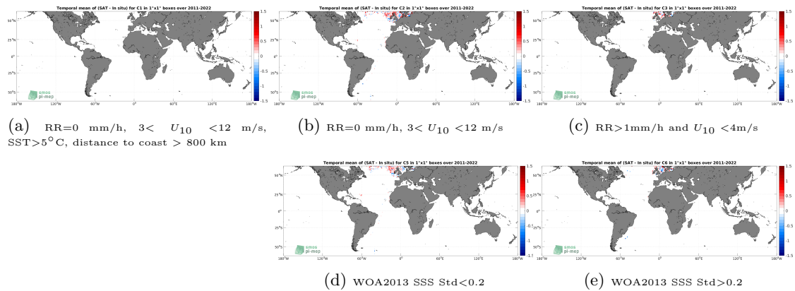
Figure 12: Temporal mean gridded over spatial boxes of size 1^\circ \times 1^\circ of \Delta SSS (SMOS SSS L4 OI v342 - Weekly (CMEMS-CATDS-LOPS) - ICES) for 5 different subdatasets corresponding to:RR=0 mm/h, 3 < U_{10} < 12 m/s, SST >5^\circ C, distance to coast > 800 km (a), RR=0 mm/h, 3 < U_{10} < 12 m/s (b), RR >1 mm/h and U_{10} < 4 m/s (c), WOA2013 SSS Std <0.2 (d), WOA2013 SSS Std >0.2 (e).
