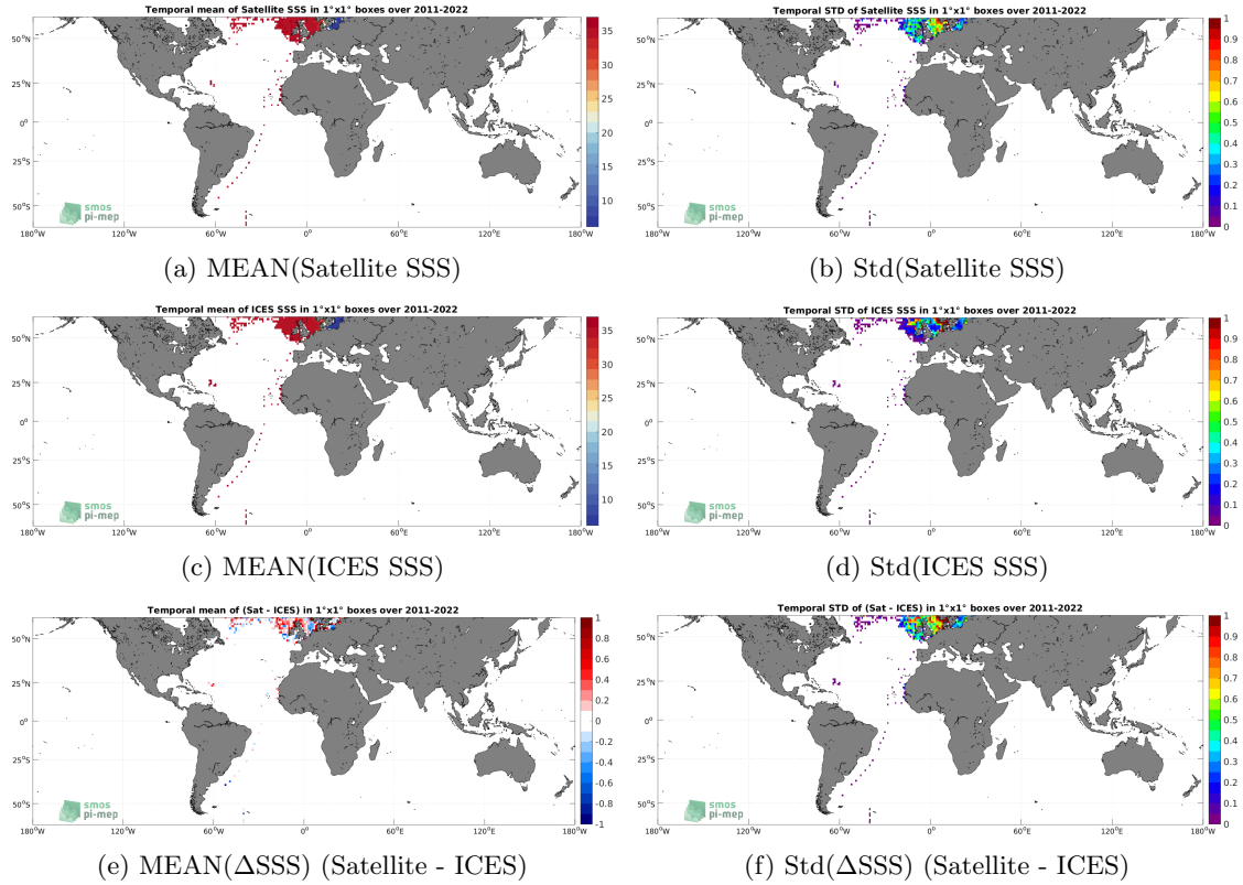
Figure 6: Temporal mean (left) and Std (right) of SSS from SMOS SSS L4 OI v342 - Weekly (CMEMS-CATDS-LOPS) (top), ICES (middle), and of \Delta SSS (Satellite - ICES). Only match-up pairs are used to generate these maps.
