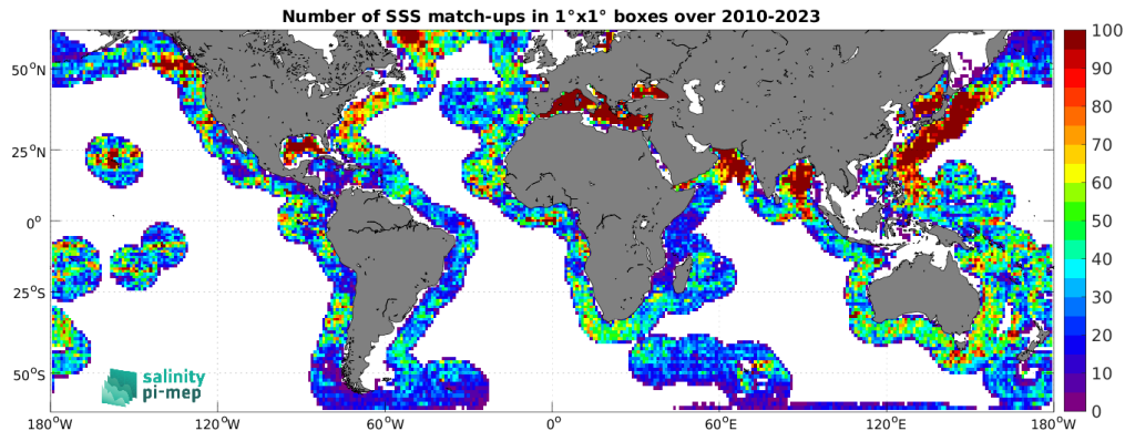
Figure 4: Number of SSS match-ups between Argo SSS and the SMOS SSS L4 OI v342 - Weekly (CMEMS-CATDS-LOPS) SSS product for the SMOS coastal zone ( <800\text{km} ) 60N-60S Pi-MEP region over 1^\circ \times 1^\circ boxes and for the full satellite product period.
