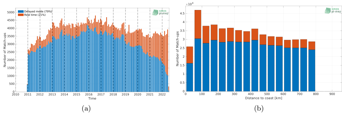
Figure 1: Number of match-ups between Argo and SMOS SSS L4 OI v342 - Weekly (CMEMS-CATDS-LOPS) SSS as a function of time (a) and as function of the distance to coast (b) over the SMOS coastal zone (<800km) 60N-60S Pi-MEP region and for the full satellite product period.
