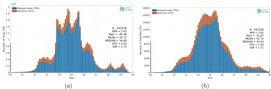
Figure 2: Histograms of SSS from Argo (a) and SMOS SSS L4 OI v342 - Weekly (CMEMS-CATDS-LOPS) (b) considering all match-up pairs per bins of 0.1 over the SMOS coastal zone (<800km) 60N-60S Pi-MEP region and for the full satellite product period.
