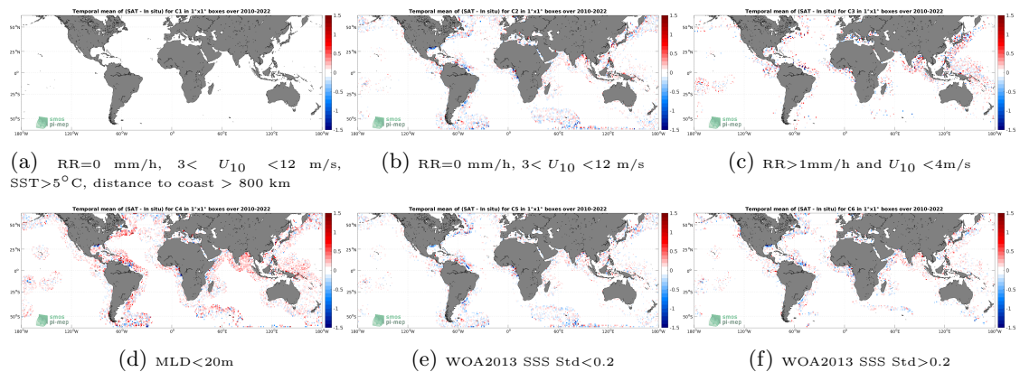
Figure 12: Temporal mean gridded over spatial boxes of size 1^\circ \times 1^\circ of \Delta SSS (SMOS SSS L4 OI v342 - Weekly (CMEMS-CATDS-LOPS) - Argo) for 6 different subdatasets corresponding to:RR=0 mm/h, 3 < U_{10} < 12 m/s, SST >5^\circ C, distance to coast > 800 km (a), RR=0 mm/h, 3 < U_{10} < 12 m/s (b), RR >1 mm/h and U_{10} < 4 m/s (c),MLD <20 m (d),WOA2013 SSS Std <0.2 (e),WOA2013 SSS Std >0.2 (f).
