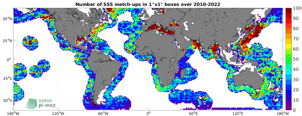
Figure 4: Number of SSS match-ups between Argo SSS and the SMOS SSS L4 OI v342 - Weekly (CMEMS-CATDS-LOPS) SSS product for the SMOS coastal zone (<800km) 60N-60S Pi-MEP region over 1^\circ \times 1^\circ boxes and for the full satellite product period.
