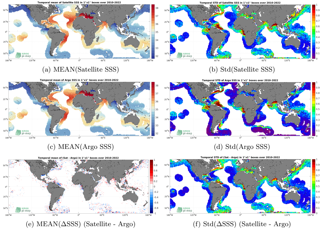
Figure 6: Temporal mean (left) and Std (right) of SSS from SMOS SSS L4 OI v342 - Weekly (CMEMS-CATDS-LOPS) (top), Argo (middle), and of \Delta SSS (Satellite - Argo). Only match-up pairs are used to generate these maps.
