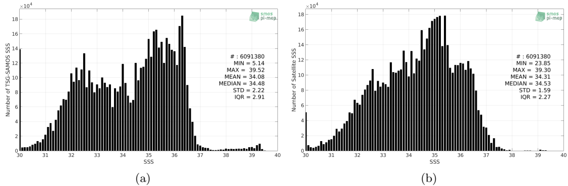
Figure 2: Histograms of SSS from TSG-SAMOS (a) and SMOS-L4-CATDS-CECOS-IFREMER-V2-WEEKLY-0.5DEG (b) considering all match-up pairs per bins of 0.1 over the SMOS coastal zone (<800km) 60N-60S Pi-MEP region and for the full satellite product period.
