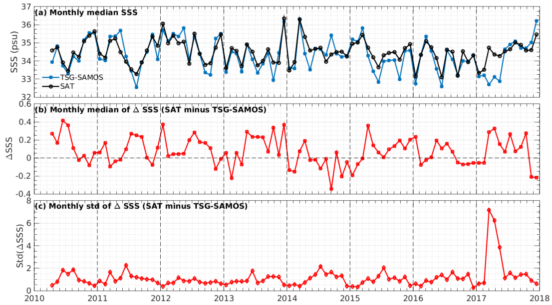
Figure 7: Time series of the monthly median SSS (top), median of \Delta SSS (Satellite - TSG-SAMOS) and Std of \Delta SSS (Satellite - TSG-SAMOS) over the SMOS coastal zone ( \geq 800 km) over the 60N-60S Pi-MEP region considering all match-ups collected by the Pi-MEP.
