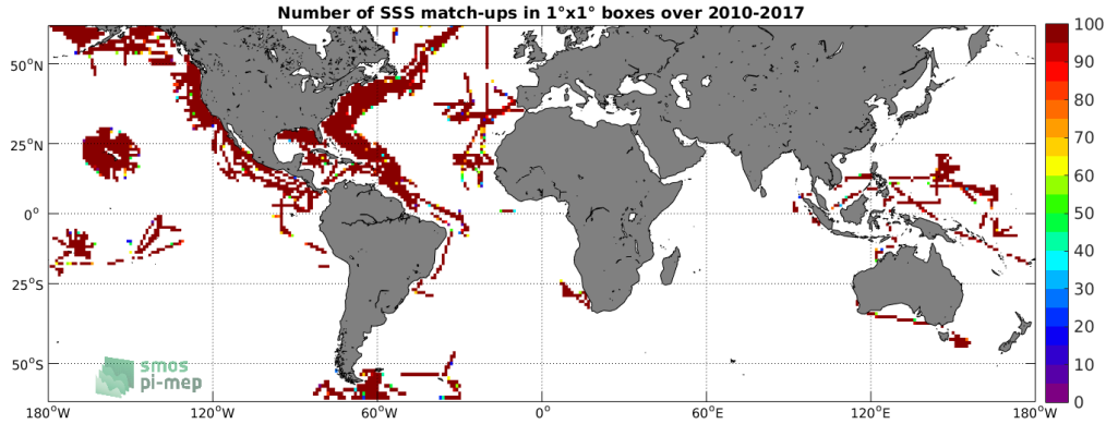
Figure 4: Number of SSS match-ups between TSG-SAMOS SSS and the SMOS-L4-CATDS-CECOS-IFREMER-V2-WEEKLY-0.5DEG SSS product for the SMOS coastal zone ( \approx 800\text{km} ) 60N-60S Pi-MEP region over 1^\circ \times 1^\circ boxes and for the full satellite product period.
