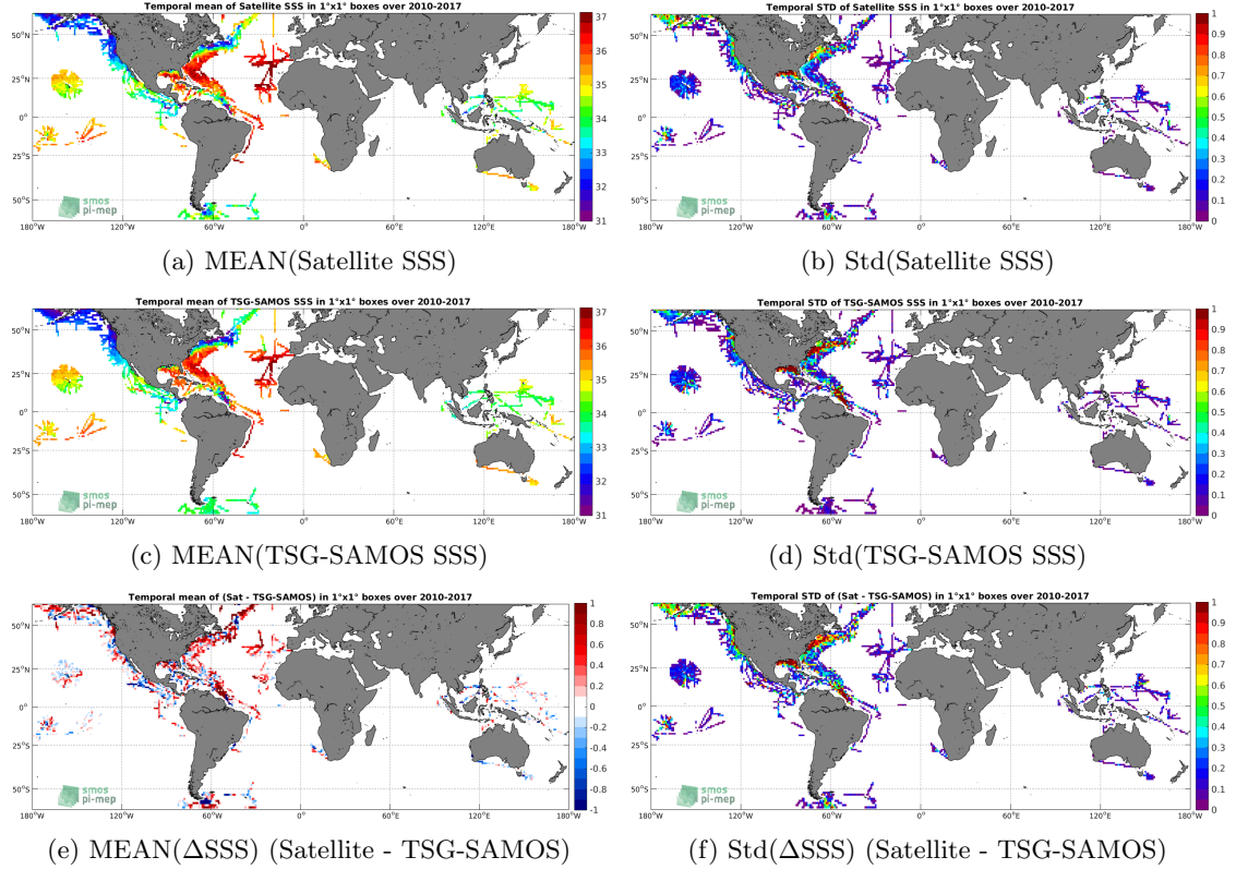
Figure 6: Temporal mean (left) and Std (right) of SSS from SMOS-L4-CATDS-CECOS-IFREMER-V2-WEEKLY-0.5DEG (top), TSG-SAMOS (middle), and of \Delta SSS (Satellite - TSG-SAMOS). Only match-up pairs are used to generate these maps.
