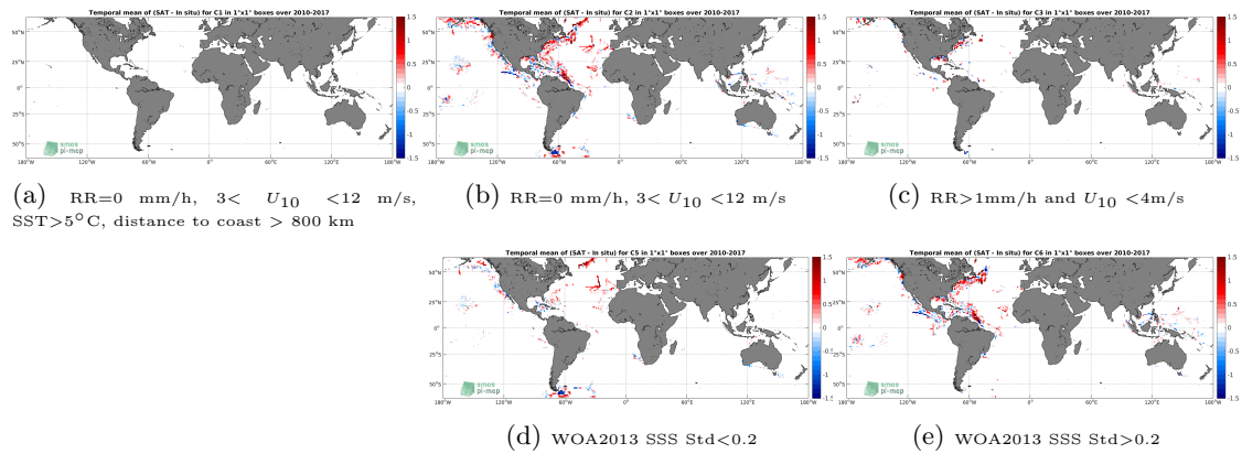
Figure 12: Temporal mean gridded over spatial boxes of size 1^\circ \times 1^\circ of \Delta SSS (SMOS-L4-CATDS-CECOS-IFREMER-V2-WEEKLY-0.5DEG - TSG-SAMOS) for 5 different subdatasets corresponding to:RR=0 mm/h, 3 < U_{10} < 12 m/s, SST >5^\circ C, distance to coast > 800 km (a), RR=0 mm/h, 3 < U_{10} < 12 m/s (b), RR >1 mm/h and U_{10} < 4 m/s (c), WOA2013 SSS Std <0.2 (d), WOA2013 SSS Std >0.2 (e).
