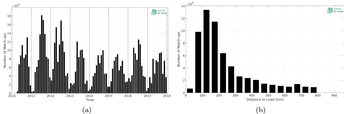
Figure 1: Number of match-ups between TSG-SAMOS and SMOS-L4-CATDS-CECOS-IFREMER-V2-WEEKLY-0.5DEG SSS as a function of time (a) and as function of the distance to coast (b) over the SMOS coastal zone ( \approx 800 km) 60N-60S Pi-MEP region and for the full satellite product period.
