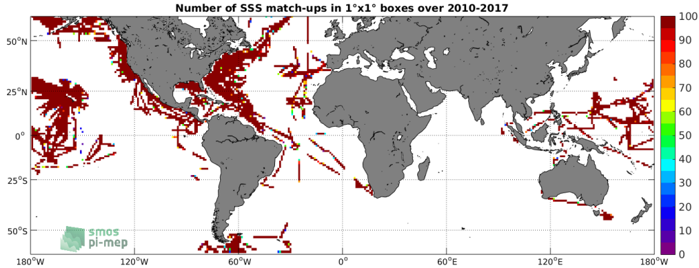
Figure 4: Number of SSS match-ups between TSG-SAMOS SSS and the SMOS-L4-CATDS-CECOS-IFREMER-V2-WEEKLY-0.5DEG SSS product for the SMOS coastal zone ( \leq 800\text{km} ) 60N-60S Pi-MEP region over 1^\circ \times 1^\circ boxes and for the full satellite product period.
