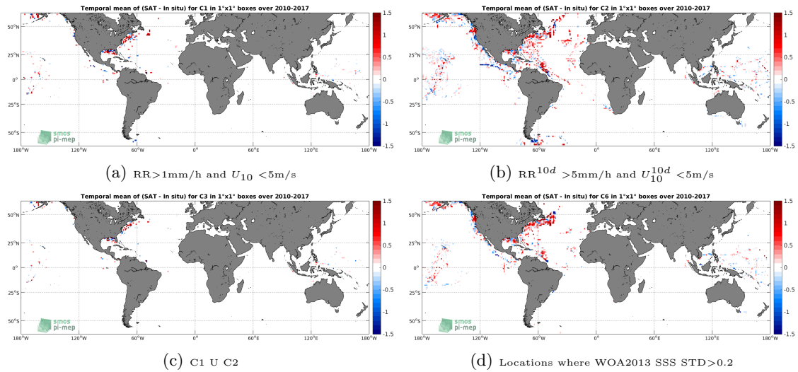
Figure 12: Temporal mean gridded over spatial boxes of size 1^\circ \times 1^\circ of \Delta SSS (SMOS-L4-CATDS-CECOS-IFREMER-V2-WEEKLY-0.5DEG - TSG-SAMOS) for 4 different subdatasets corresponding to: RR > 1\text{mm/h} and U_{10} < 5\text{m/s} (a), RR^{10d} > 5\text{mm/h} and U_{10}^{10d} < 5\text{m/s} (b), C1 U C2 (c), Locations where WOA2013 SSS STD > 0.2 (d).
