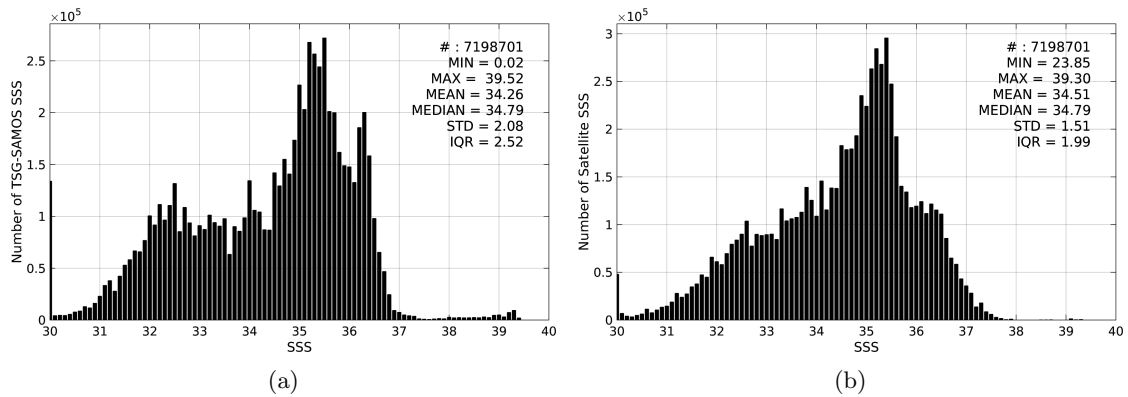
Figure 2: Histograms of SSS from TSG-SAMOS (a) and SMOS-L4-CATDS-CECOS-IFREMER-V2-WEEKLY-0.5DEG (b) considering all match-up pairs per bins of 0.1 over the SMOS coastal zone ( \approx 800\text{km} ) 60N-60S Pi-MEP region and for the full satellite product period.
