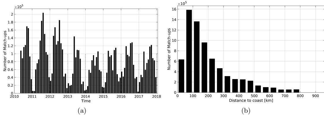
Figure 1: Number of match-ups between TSG-SAMOS and SMOS-L4-CATDS-CECOS-IFREMER-V2-WEEKLY-0.5DEG SSS as a function of time (a) and as function of the distance to coast (b) over the SMOS coastal zone ( \pm 800 km) 60N-60S Pi-MEP region and for the full satellite product period.
