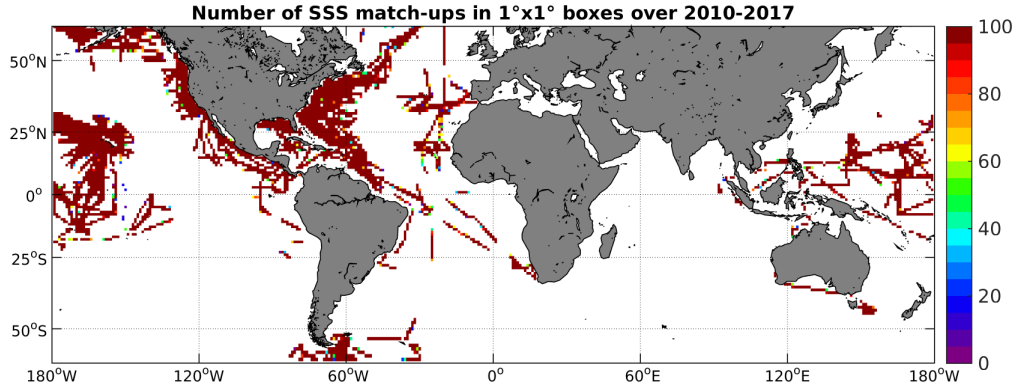
Figure 4: Number of SSS match-ups between TSG-SAMOS SSS and the SMOS-L4-CATDS-CECOS-IFREMER-V2-WEEKLY-0.5DEG SSS product for the SMOS coastal zone ( \delta 800\text{km} ) 60N-60S Pi-MEP region over 1°x1° boxes and for the full satellite product period.
