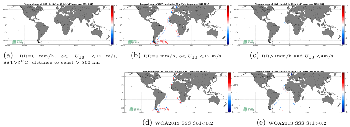
Figure 12: Temporal mean gridded over spatial boxes of size 1^\circ \times 1^\circ of \Delta SSS (SMOS L4 v2 Weekly (CATDS-CECOS-IFREMER) - TSG (Polarstern)) for 5 different subdatasets corresponding to:RR=0 mm/h, 3 < U_{10} < 12 m/s, SST > 5^\circ\text{C} , distance to coast > 800 km (a), RR=0 mm/h, 3 < U_{10} < 12 m/s (b), RR > 1 mm/h and U_{10} < 4 m/s (c), WOA2013 SSS Std < 0.2 (d), WOA2013 SSS Std > 0.2 (e).
