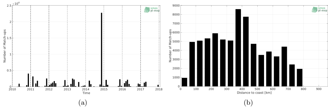
Figure 1: Number of match-ups between TSG (Polarstern) and SMOS L4 v2 Weekly (CATDS-CECOS-IFREMER) SSS as a function of time (a) and as function of the distance to coast (b) over the SMOS coastal zone (<800km) 60N-60S Pi-MEP region and for the full satellite product period.
