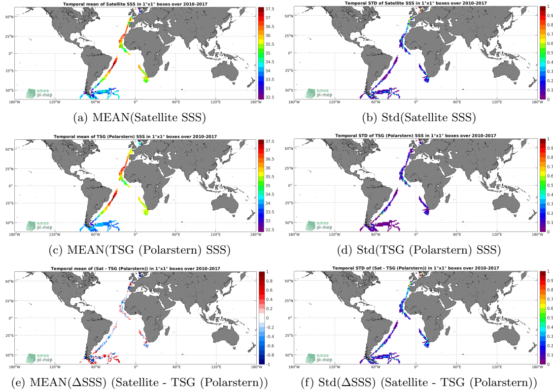
Figure 6: Temporal mean (left) and Std (right) of SSS from SMOS L4 v2 Weekly (CATDS-CECOS-IFREMER) (top), TSG (Polarstern) (middle), and of \Delta SSS (Satellite - TSG (Polarstern)). Only match-up pairs are used to generate these maps.
