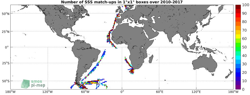
Figure 4: Number of SSS match-ups between TSG (Polarstern) SSS and the SMOS L4 v2 Weekly (CATDS-CECOS-IFREMER) SSS product for the SMOS coastal zone (<800km) 60N-60S Pi-MEP region over 1^\circ \times 1^\circ boxes and for the full satellite product period.
