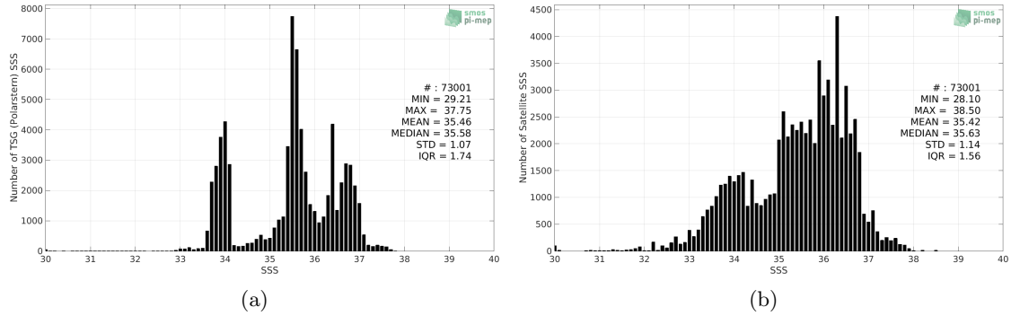
Figure 2: Histograms of SSS from TSG (Polarstern) (a) and SMOS L4 v2 Weekly (CATDS-CECOS-IFREMER) (b) considering all match-up pairs per bins of 0.1 over the SMOS coastal zone (<800km) 60N-60S Pi-MEP region and for the full satellite product period.
