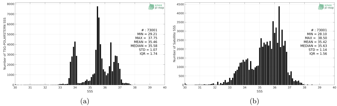
Figure 2: Histograms of SSS from TSG-POLARSTERN (a) and SMOS-L4-CATDS-CECOS-IFREMER-V2-WEEKLY-0.5DEG (b) considering all match-up pairs per bins of 0.1 over the SMOS coastal zone (<800km) 60N-60S Pi-MEP region and for the full satellite product period.
