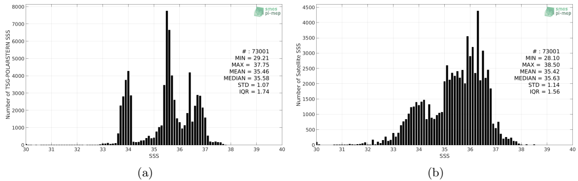
Figure 2: Histograms of SSS from TSG-POLARSTERN (a) and SMOS-L4-CATDS-CECOS-IFREMER-V2-WEEKLY-0.5DEG (b) considering all match-up pairs per bins of 0.1 over the SMOS coastal zone ( \pm 800\text{km} ) 60N-60S Pi-MEP region and for the full satellite product period.
