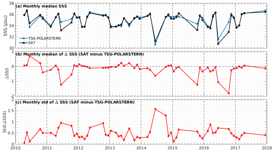
Figure 7: Time series of the monthly median SSS (top), median of \Delta SSS (Satellite - TSG-POLARSTERN) and Std of \Delta SSS (Satellite - TSG-POLARSTERN) over the SMOS coastal zone ( \pm 800\text{km} ) 60N-60S Pi-MEP region considering all match-ups collected by the Pi-MEP.
