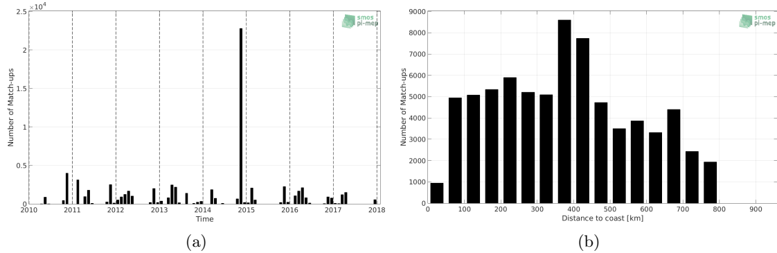
Figure 1: Number of match-ups between TSG-POLARSTERN and SMOS-L4-CATDS-CECOS-IFREMER-V2-WEEKLY-0.5DEG SSS as a function of time (a) and as function of the distance to coast (b) over the SMOS coastal zone ( \approx 800 km) 60N-60S Pi-MEP region and for the full satellite product period.
