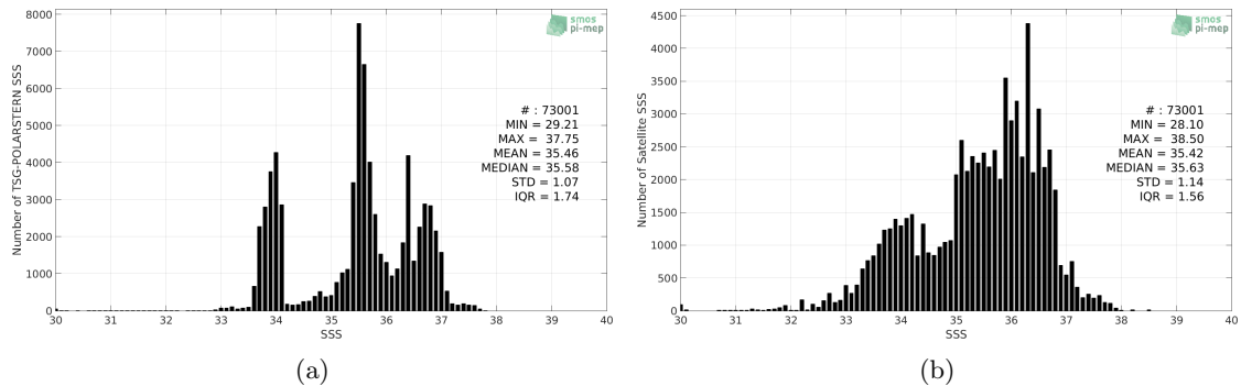
Figure 2: Histograms of SSS from TSG-POLARSTERN (a) and SMOS-L4-CATDS-CECOS-IFREMER-V2-WEEKLY-0.5DEG (b) considering all match-up pairs per bins of 0.1 over the SMOS coastal zone ( \approx 800 km) 60N-60S Pi-MEP region and for the full satellite product period.
