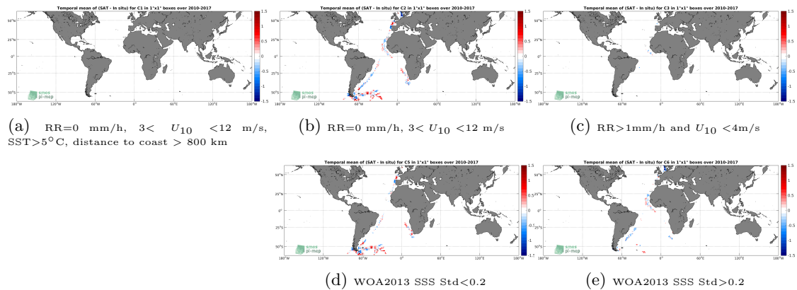
Figure 12: Temporal mean gridded over spatial boxes of size 1^\circ \times 1^\circ of \Delta SSS (SMOS-L4-CATDS-CECOS-IFREMER-V2-WEEKLY-0.5DEG - TSG-POLARSTERN) for 5 different subdatasets corresponding to:RR=0 mm/h, 3 < U_{10} < 12 m/s, SST >5^\circ C, distance to coast > 800 km (a), RR=0 mm/h, 3 < U_{10} < 12 m/s (b), RR >1 mm/h and U_{10} < 4 m/s (c), WOA2013 SSS Std <0.2 (d), WOA2013 SSS Std >0.2 (e).
