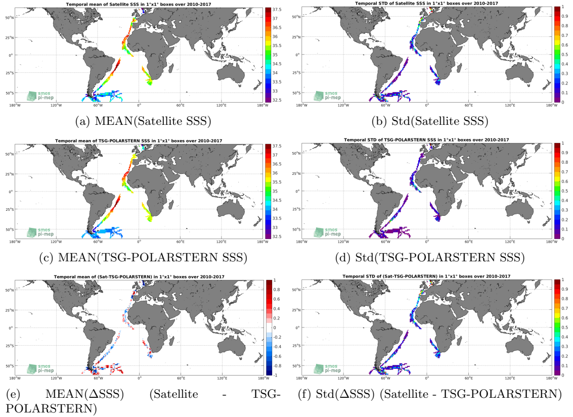
Figure 6: Temporal mean (left) and Std (right) of SSS from SMOS-L4-CATDS-CECOS-IFREMER-V2-WEEKLY-0.5DEG (top), TSG-POLARSTERN (middle), and of \Delta SSS (Satellite - TSG-POLARSTERN). Only match-up pairs are used to generate these maps.
