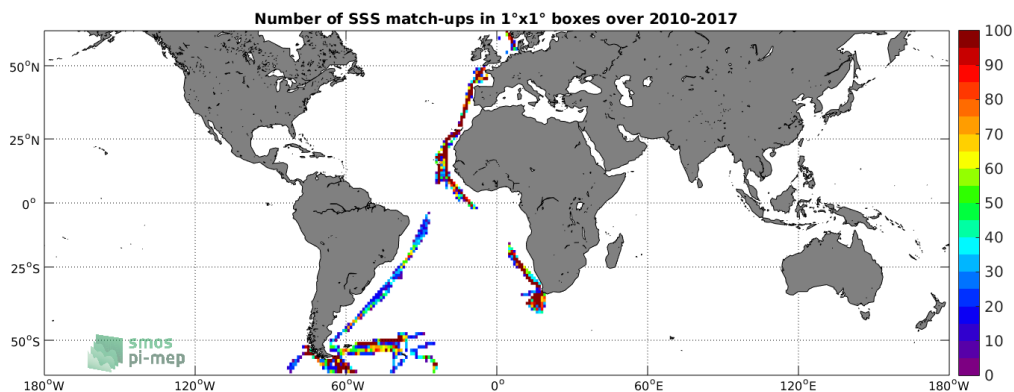
Figure 4: Number of SSS match-ups between TSG-POLARSTERN SSS and the SMOS-L4-CATDS-CECOS-IFREMER-V2-WEEKLY-0.5DEG SSS product for the SMOS coastal zone ( \pm 800\text{km} ) 60N-60S Pi-MEP region over 1^\circ \times 1^\circ boxes and for the full satellite product period.
