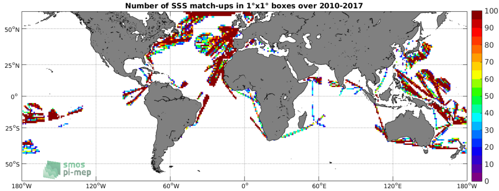
Figure 4: Number of SSS match-ups between TSG-LEGOS-DM SSS and the SMOS-L4-CATDS-CECOS-IFREMER-V2-WEEKLY-0.5DEG SSS product for the SMOS coastal zone ( \approx 800\text{km} ) 60N-60S Pi-MEP region over 1^\circ \times 1^\circ boxes and for the full satellite product period.
