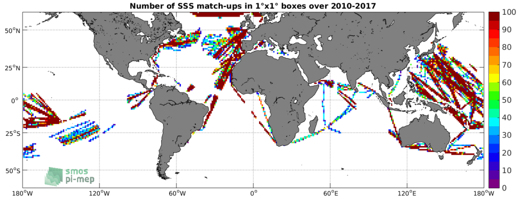
Figure 4: Number of SSS match-ups between TSG-LEGOS-DM SSS and the SMOS-L4-CATDS-CECOS-IFREMER-V2-WEEKLY-0.5DEG SSS product for the SMOS coastal zone ( \leq 800\text{km} ) 60N-60S Pi-MEP region over 1^\circ \times 1^\circ boxes and for the full satellite product period.
