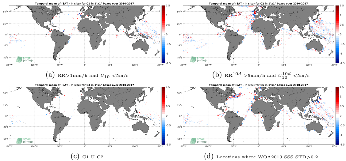
Figure 12: Temporal mean gridded over spatial boxes of size 1^\circ \times 1^\circ of \Delta SSS (SMOS-L4-CATDS-CECOS-IFREMER-V2-WEEKLY-0.5DEG - TSG-LEGOS-DM) for 4 different subdatasets corresponding to: RR > 1\text{mm/h} and U_{10} < 5\text{m/s} (a), RR^{10d} > 5\text{mm/h} and U_{10}^{10d} < 5\text{m/s} (b), C1 U C2 (c), Locations where WOA2013 SSS STD > 0.2 (d).
