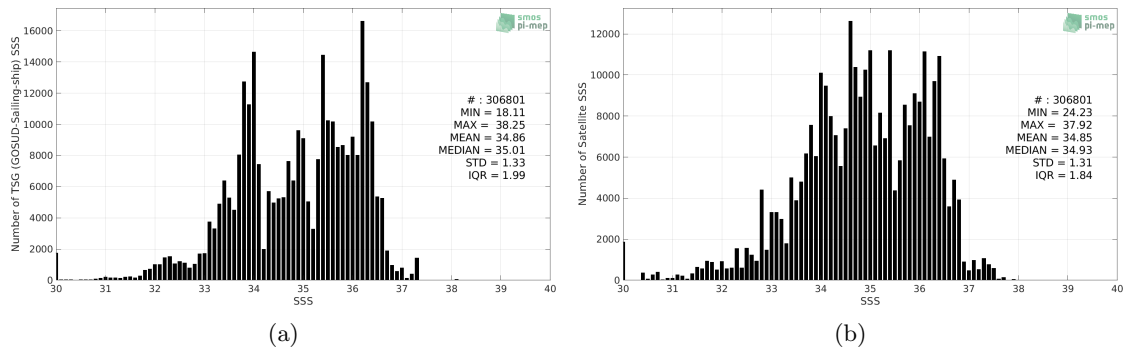
Figure 2: Histograms of SSS from TSG (GOSUD-Sailing-ship) (a) and SMOS L4 v2 Weekly (CATDS-CECOS-IFREMER) (b) considering all match-up pairs per bins of 0.1 over the SMOS coastal zone (<800km) 60N-60S Pi-MEP region and for the full satellite product period.
