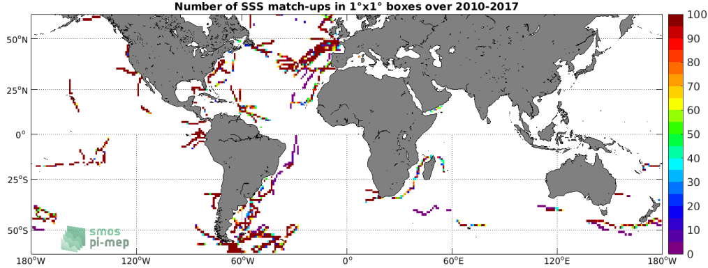
Figure 4: Number of SSS match-ups between TSG (GOSUD-Sailing-ship) SSS and the SMOS L4 v2 Weekly (CATDS-CECOS-IFREMER) SSS product for the SMOS coastal zone (<800km) 60N-60S Pi-MEP region over 1^\circ \times 1^\circ boxes and for the full satellite product period.
