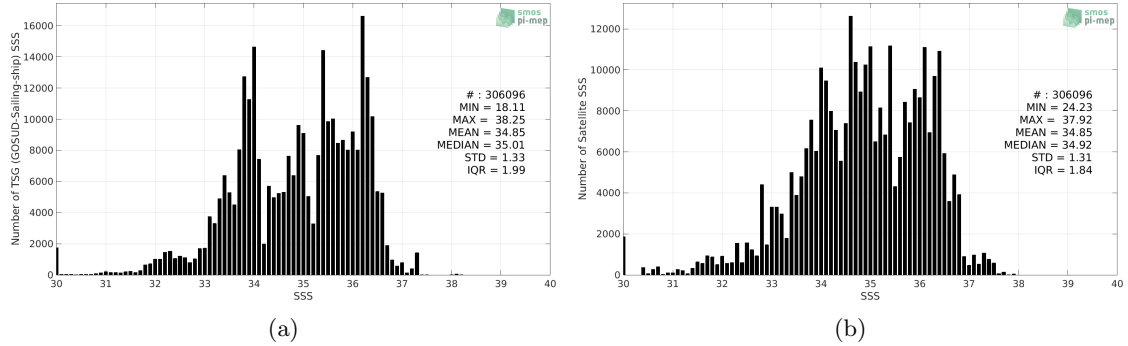
Figure 2: Histograms of SSS from TSG (GOSUD-Sailing-ship) (a) and SMOS L4 v2 Weekly (CATDS-CECOS-IFREMER) (b) considering all match-up pairs per bins of 0.1 over the SMOS coastal zone (<800km) 60N-60S Pi-MEP region and for the full satellite product period.
