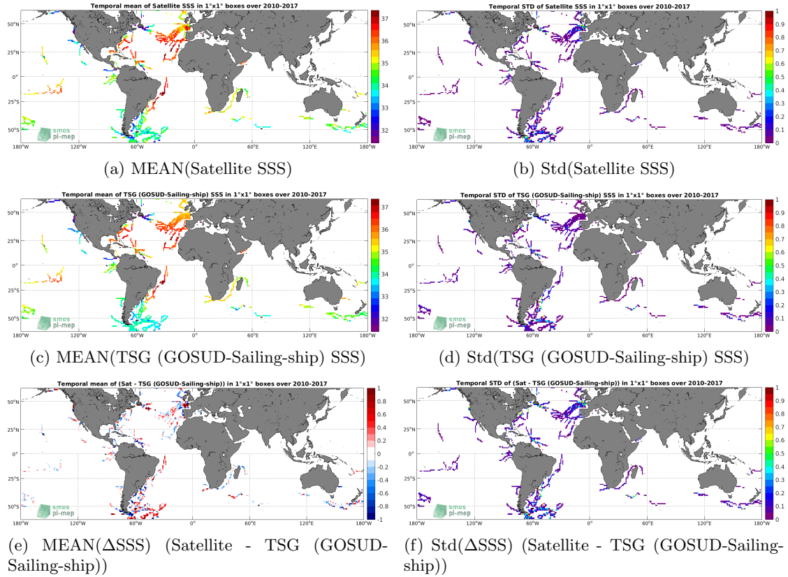
Figure 6: Temporal mean (left) and Std (right) of SSS from SMOS L4 v2 Weekly (CATDS-CECOS-IFREMER) (top), TSG (GOSUD-Sailing-ship) (middle), and of \Delta SSS (Satellite - TSG (GOSUD-Sailing-ship)). Only match-up pairs are used to generate these maps.
