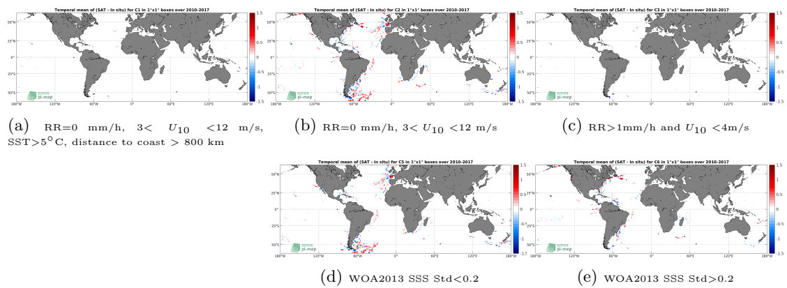
Figure 12: Temporal mean gridded over spatial boxes of size 1^\circ \times 1^\circ of \Delta SSS (SMOS L4 v2 Weekly (CATDS-CECOS-IFREMER) - TSG (GOSUD-Sailing-ship)) for 5 different subdatasets corresponding to: RR=0 mm/h, 3 < U_{10} < 12 m/s, SST > 5°C, distance to coast > 800 km (a), RR=0 mm/h, 3 < U_{10} < 12 m/s (b), RR > 1mm/h and U_{10} < 4 m/s (c), WOA2013 SSS Std < 0.2 (d), WOA2013 SSS Std > 0.2 (e).
