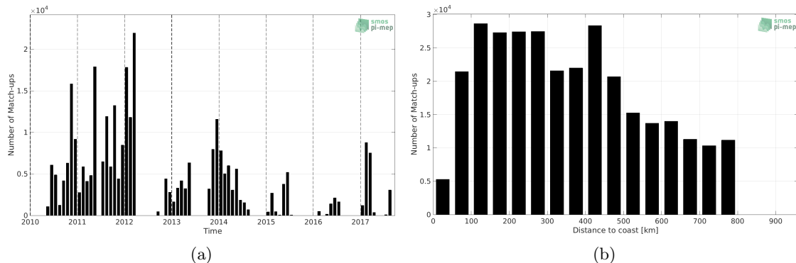
Figure 1: Number of match-ups between TSG (GOSUD-Sailing-ship) and SMOS L4 v2 Weekly (CATDS-CECOS-IFREMER) SSS as a function of time (a) and as function of the distance to coast (b) over the SMOS coastal zone (<800km) 60N-60S Pi-MEP region and for the full satellite product period.
