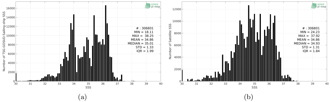
Figure 2: Histograms of SSS from TSG-GOSUD-Sailing-ship (a) and SMOS-L4-CATDS-CECOS-IFREMER-V2-WEEKLY-0.5DEG (b) considering all match-up pairs per bins of 0.1 over the SMOS coastal zone (<800km) 60N-60S Pi-MEP region and for the full satellite product period.
