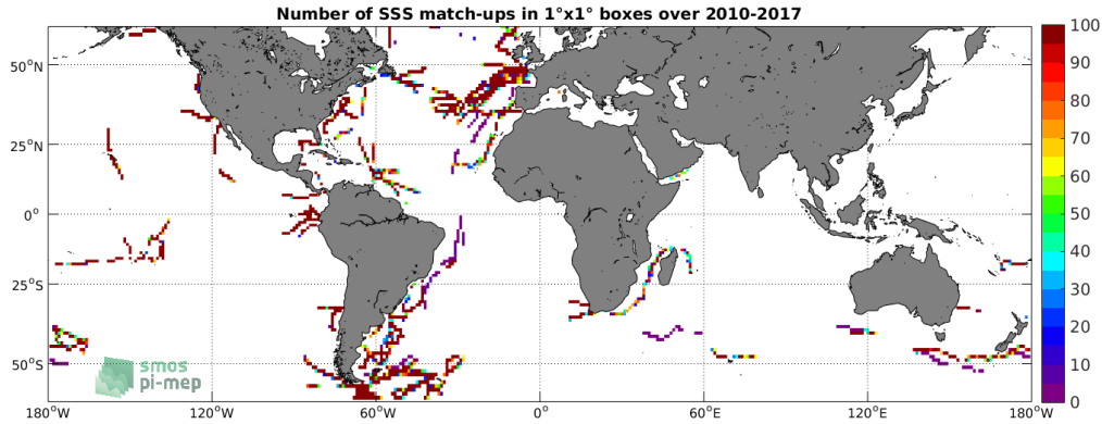
Figure 4: Number of SSS match-ups between TSG-GOSUD-Sailing-ship SSS and the SMOS-L4-CATDS-CECOS-IFREMER-V2-WEEKLY-0.5DEG SSS product for the SMOS coastal zone (<800km) 60N-60S Pi-MEP region over 1^{\circ} \times 1^{\circ} boxes and for the full satellite product period.
