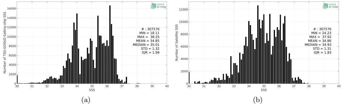
Figure 2: Histograms of SSS from TSG-GOSUD-Sailing-ship (a) and SMOS-L4-CATDS-CECOS-IFREMER-V2-WEEKLY-0.5DEG (b) considering all match-up pairs per bins of 0.1 over the SMOS coastal zone ( \pm 800\text{km} ) 60N-60S Pi-MEP region and for the full satellite product period.
