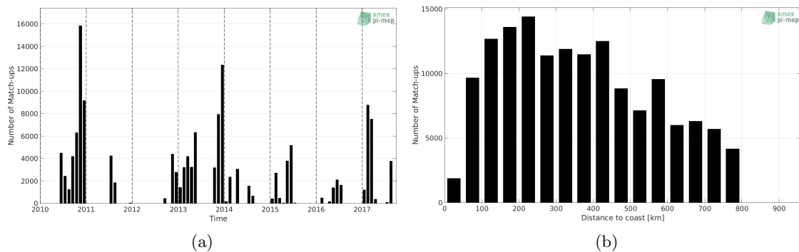
Figure 1: Number of match-ups between TSG-GOSUD-Sailing-ship and SMOS-L4-CATDS-CECOS-IFREMER-V2-WEEKLY-0.5DEG SSS as a function of time (a) and as function of the distance to coast (b) over the SMOS coastal zone ( \pm 800 km) 60N-60S Pi-MEP region and for the full satellite product period.
