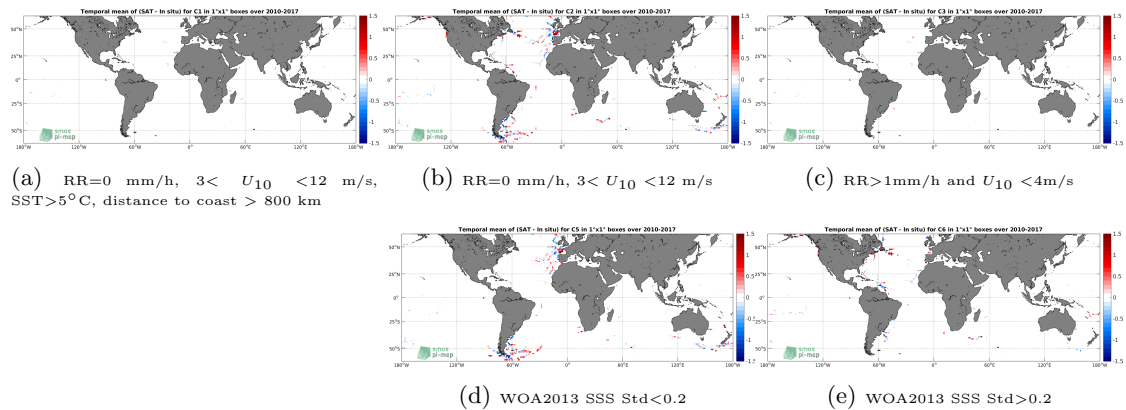
Figure 12: Temporal mean gridded over spatial boxes of size 1^\circ \times 1^\circ of \Delta SSS (SMOS-L4-CATDS-CECOS-IFREMER-V2-WEEKLY-0.5DEG - TSG-GOSUD-Sailing-ship) for 5 different subdatasets corresponding to:RR=0 mm/h, 3 < U_{10} < 12 m/s, SST >5^\circ C, distance to coast > 800 km (a), RR=0 mm/h, 3 < U_{10} < 12 m/s (b), RR >1 mm/h and U_{10} < 4 m/s (c), WOA2013 SSS Std <0.2 (d), WOA2013 SSS Std >0.2 (e).
