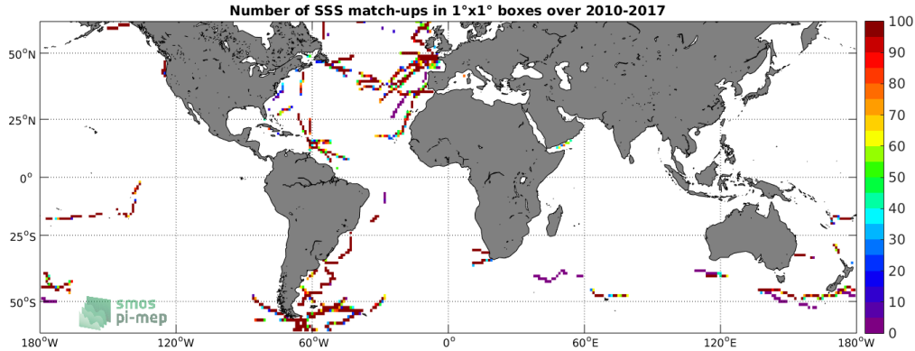
Figure 4: Number of SSS match-ups between TSG-GOSUD-Sailing-ship SSS and the SMOS-L4-CATDS-CECOS-IFREMER-V2-WEEKLY-0.5DEG SSS product for the SMOS coastal zone ( \approx 800\text{km} ) 60N-60S Pi-MEP region over 1^\circ \times 1^\circ boxes and for the full satellite product period.
