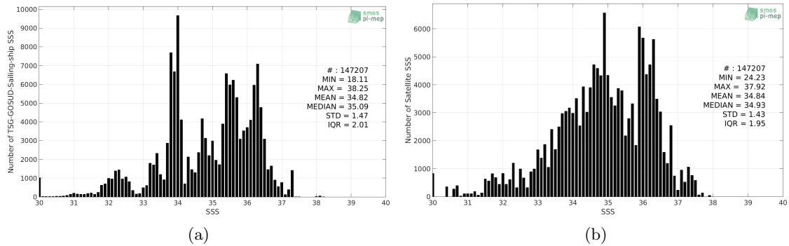
Figure 2: Histograms of SSS from TSG-GOSUD-Sailing-ship (a) and SMOS-L4-CATDS-CECOS-IFREMER-V2-WEEKLY-0.5DEG (b) considering all match-up pairs per bins of 0.1 over the SMOS coastal zone ( \approx 800\text{km} ) 60N-60S Pi-MEP region and for the full satellite product period.
