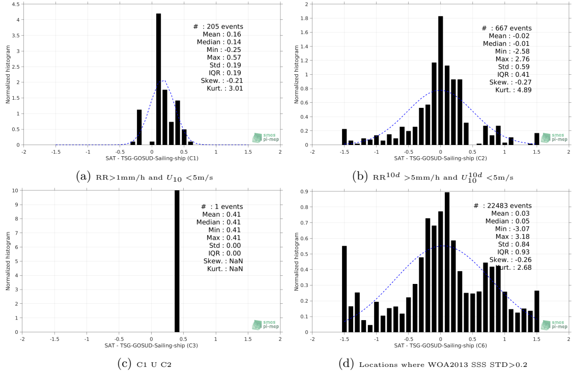
Figure 13: Normalized histogram of \Delta SSS (SMOS-L4-CATDS-CECOS-IFREMER-V2-WEEKLY-0.5DEG - TSG-GOSUD-Sailing-ship) for 6 different subdatasets corresponding to: RR > 1mm/h and U_{10} < 5 m/s (a), RR^{10d} > 5 mm/h and U_{10}^{10d} < 5 m/s (b), C1 U C2 (c), Locations where WOA2013 SSS STD > 0.2 (d).
