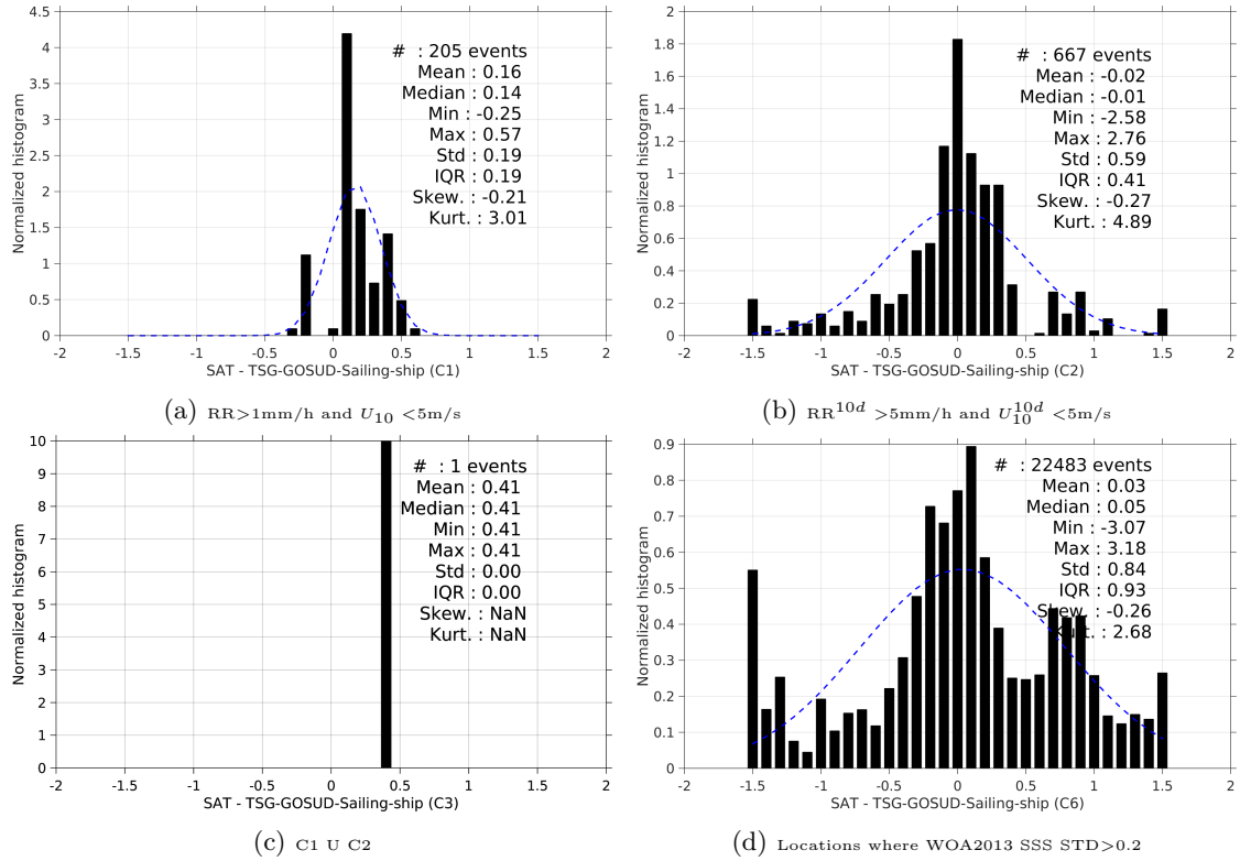
Figure 13: Normalized histogram of \Delta\text{SSS} (SMOS-L4-CATDS-CECOS-IFREMER-V2-WEEKLY-0.5DEG - TSG-GOSUD-Sailing-ship) for 6 different subdatasets corresponding to: RR > 1mm/h and U_{10} < 5\text{m/s} (a), RR^{10d} > 5\text{mm/h} and U_{10}^{10d} < 5\text{m/s} (b), C1 U C2 (c), Locations where WOA2013 SSS STD > 0.2 (d).
