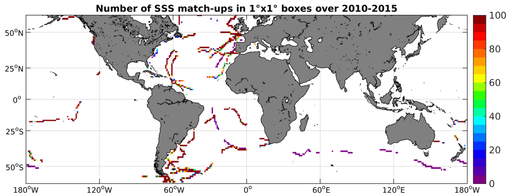
Figure 4: Number of SSS match-ups between TSG-GOSUD-Sailing-ship SSS and the SMOS-L4-CATDS-CECOS-IFREMER-V2-WEEKLY-0.5DEG SSS product for the SMOS coastal zone ( \pm 800\text{km} ) 60N-60S Pi-MEP region over 1^\circ \times 1^\circ boxes and for the full satellite product period.
