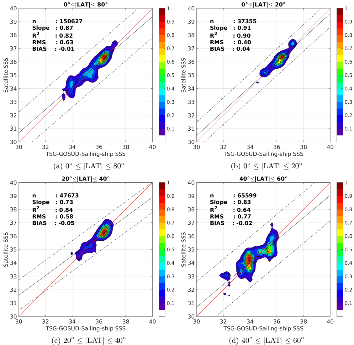
Figure 9: Contour maps of the concentration of SMOS-L4-CATDS-CECOS-IFREMER-V2-WEEKLY-0.5DEG SSS (y-axis) versus TSG-GOSUD-Sailing-ship SSS (x-axis) at match-up pairs for different latitude bands. For each plot, the red line shows x=y . The black thin and dashed lines indicate a linear fit through the data cloud and the \pm 95\% confidence levels, respectively. The number match-up pairs n , the slope and R^2 coefficient of the linear fit, the root mean square (RMS) and the mean bias between satellite and in situ data are indicated for each latitude band in each plots.
