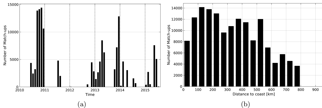
Figure 1: Number of match-ups between TSG-GOSUD-Sailing-ship and SMOS-L4-CATDS-CECOS-IFREMER-V2-WEEKLY-0.5DEG SSS as a function of time (a) and as function of the distance to coast (b) over the SMOS coastal zone ( \pm 800 km) 60N-60S Pi-MEP region and for the full satellite product period.
