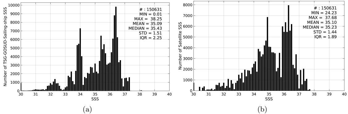
Figure 2: Histograms of SSS from TSG-GOSUD-Sailing-ship (a) and SMOS-L4-CATDS-CECOS-IFREMER-V2-WEEKLY-0.5DEG (b) considering all match-up pairs per bins of 0.1 over the SMOS coastal zone ( \approx 800\text{km} ) 60N-60S Pi-MEP region and for the full satellite product period.
