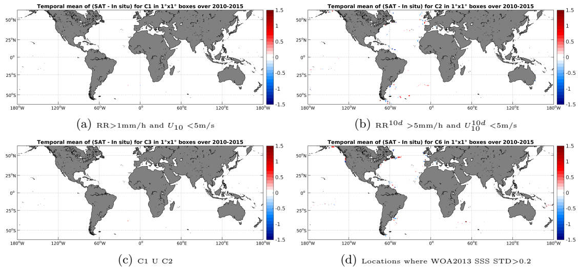
Figure 12: Temporal mean gridded over spatial boxes of size 1^\circ \times 1^\circ of \Delta SSS (SMOS-L4-CATDS-CECOS-IFREMER-V2-WEEKLY-0.5DEG - TSG-GOSUD-Sailing-ship) for 4 different subdatasets corresponding to: RR > 1\text{mm/h} and U_{10} < 5\text{m/s} (a), RR^{10d} > 5\text{mm/h} and U_{10}^{10d} < 5\text{m/s} (b), C1 U C2 (c), Locations where WOA2013 SSS STD > 0.2 (d).
