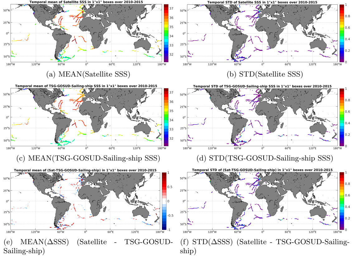
Figure 6: Temporal mean (left) and STD (right) of SSS from SMOS-L4-CATDS-CECOS-IFREMER-V2-WEEKLY-0.5DEG (top), TSG-GOSUD-Sailing-ship (middle), and of \Delta SSS (Satellite - TSG-GOSUD-Sailing-ship). Only match-up pairs are used to generate these maps.
