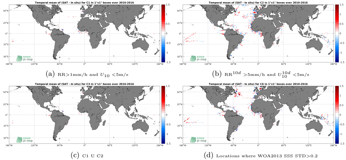
Figure 12: Temporal mean gridded over spatial boxes of size 1^\circ \times 1^\circ of \Delta SSS (SMOS-L4-CATDS-CECOS-IFREMER-V2-WEEKLY-0.5DEG - TSG-GOSUD-Research-vessel) for 4 different sub-datasets corresponding to: RR > 1mm/h and U_{10} < 5\text{m/s} (a), RR^{10d} > 5\text{mm/h} and U_{10}^{10d} < 5\text{m/s} (b), C1 U C2 (c), Locations where WOA2013 SSS STD > 0.2 (d).
