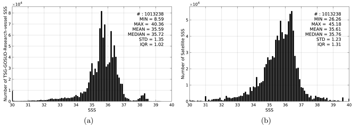
Figure 2: Histograms of SSS from TSG-GOSUD-Research-vessel (a) and SMOS-L4-CATDS-CECOS-IFREMER-V2-WEEKLY-0.5DEG (b) considering all match-up pairs per bins of 0.1 over the SMOS coastal zone ( \pm 800\text{km} ) 60N-60S Pi-MEP region and for the full satellite product period.
