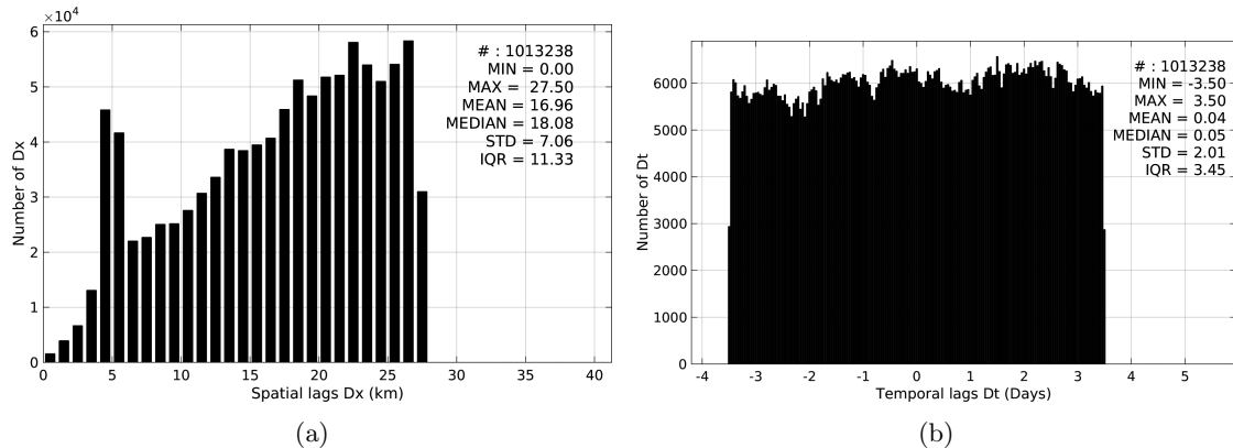
Figure 5: Histograms of the spatial (a) and temporal (b) lags between the time of the TSG-GOSUD-Research-vessel measurements and the date of the corresponding SMOS-L4-CATDS-CECOS-IFREMER-V2-WEEKLY-0.5DEG SSS product.
