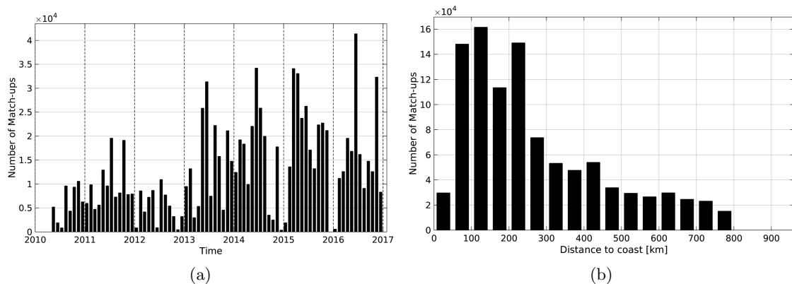
Figure 1: Number of match-ups between TSG-GOSUD-Research-vessel and SMOS-L4-CATDS-CECOS-IFREMER-V2-WEEKLY-0.5DEG SSS as a function of time (a) and as function of the distance to coast (b) over the SMOS coastal zone ( \pm 800 km) 60N-60S Pi-MEP region and for the full satellite product period.
