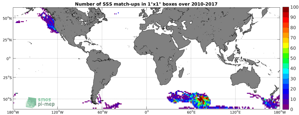
Figure 4: Number of SSS match-ups between Sea mammals SSS and the SMOS-L4-CATDS-CECOS-IFREMER-V2-WEEKLY-0.5DEG SSS product for the SMOS coastal zone (<800km) 60N-60S Pi-MEP region over 1^{\circ} \times 1^{\circ} boxes and for the full satellite product period.
