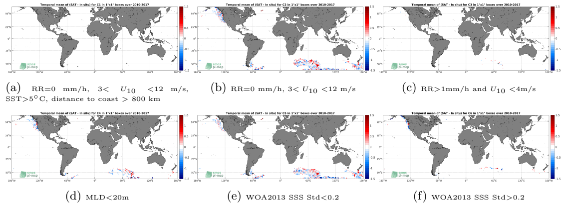
Figure 12: Temporal mean gridded over spatial boxes of size 1^{\circ}\times 1^{\circ} of \Delta\text{SSS} (SMOS-L4-CATDS-CECOS-IFREMER-V2-WEEKLY-0.5DEG - Sea mammals) for 6 different subdatasets corresponding to:RR=0 mm/h, 3 < U_{10} < 12 m/s, SST >5^{\circ}\text{C} , distance to coast > 800 km (a), RR=0 mm/h, 3 < U_{10} < 12 m/s (b), RR >1\text{mm/h} and U_{10} < 4\text{m/s} (c),MLD <20\text{m} (d),WOA2013 SSS Std <0.2 (e),WOA2013 SSS Std >0.2 (f).
