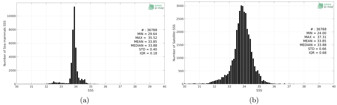
Figure 2: Histograms of SSS from Sea mammals (a) and SMOS-L4-CATDS-CECOS-IFREMER-V2-WEEKLY-0.5DEG (b) considering all match-up pairs per bins of 0.1 over the SMOS coastal zone (<800km) 60N-60S Pi-MEP region and for the full satellite product period.
