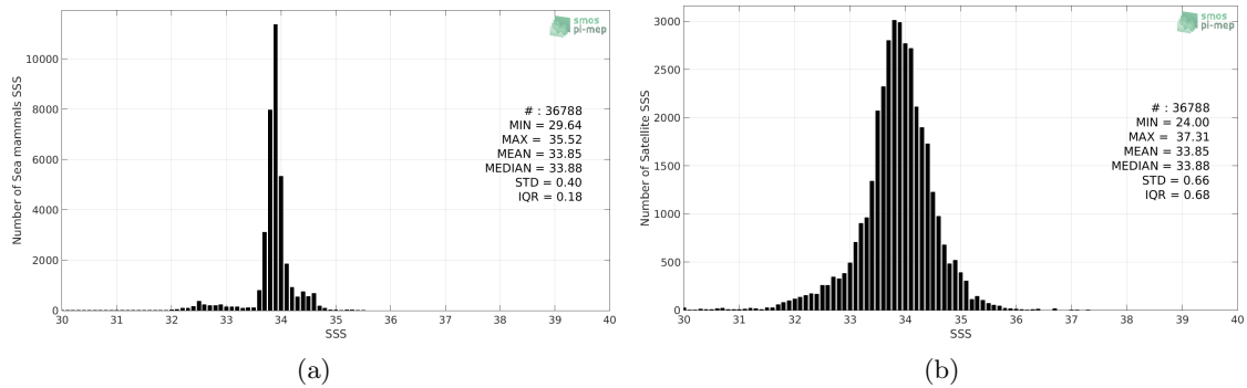
Figure 2: Histograms of SSS from Sea mammals (a) and SMOS-L4-CATDS-CECOS-IFREMER-V2-WEEKLY-0.5DEG (b) considering all match-up pairs per bins of 0.1 over the SMOS coastal zone ( \approx 800\text{km} ) 60N-60S Pi-MEP region and for the full satellite product period.
