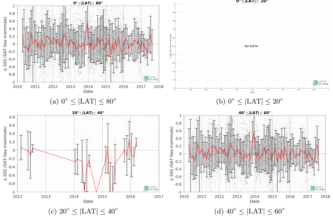
Figure 10: Monthly median (red curves) of \Delta SSS (Satellite - Sea mammals) and \pm 1 Std (black vertical thick bars) as function of time for all the collected Pi-MEP match-up pairs estimated over the SMOS coastal zone ( \approx 800\text{km} ) 60^\circ\text{N} - 60^\circ\text{S} Pi-MEP region and for the full satellite product period are shown for different latitude bands: (a) 80^\circ\text{S} - 80^\circ\text{N} , (b) 20^\circ\text{S} - 20^\circ\text{N} , (c) 40^\circ\text{S} - 20^\circ\text{S} and 20^\circ\text{N} - 40^\circ\text{N} and (d) 60^\circ\text{S} - 40^\circ\text{S} and 40^\circ\text{N} - 60^\circ\text{N} .
