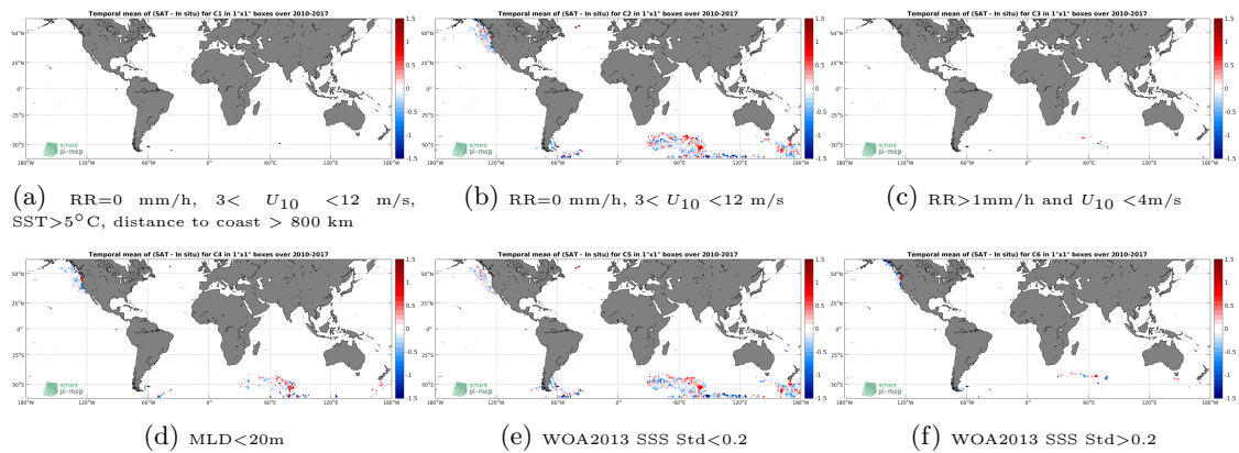
Figure 12: Temporal mean gridded over spatial boxes of size 1^\circ \times 1^\circ of \Delta SSS (SMOS-L4-CATDS-CECOS-IFREMER-V2-WEEKLY-0.5DEG - Sea mammals) for 6 different subdatasets corresponding to:RR=0 mm/h, 3 < U_{10} < 12 m/s, SST >5^\circ C, distance to coast > 800 km (a), RR=0 mm/h, 3 < U_{10} < 12 m/s (b), RR >1 mm/h and U_{10} < 4 m/s (c),MLD <20 m (d),WOA2013 SSS Std <0.2 (e),WOA2013 SSS Std >0.2 (f).
