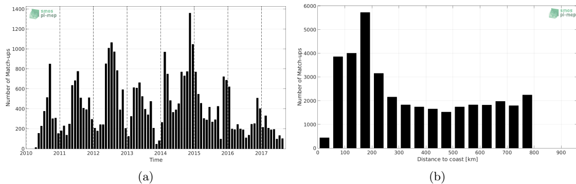
Figure 1: Number of match-ups between Sea mammals and SMOS-L4-CATDS-CECOS-IFREMER-V2-WEEKLY-0.5DEG SSS as a function of time (a) and as function of the distance to coast (b) over the SMOS coastal zone ( \leq 800 km) 60N-60S Pi-MEP region and for the full satellite product period.
