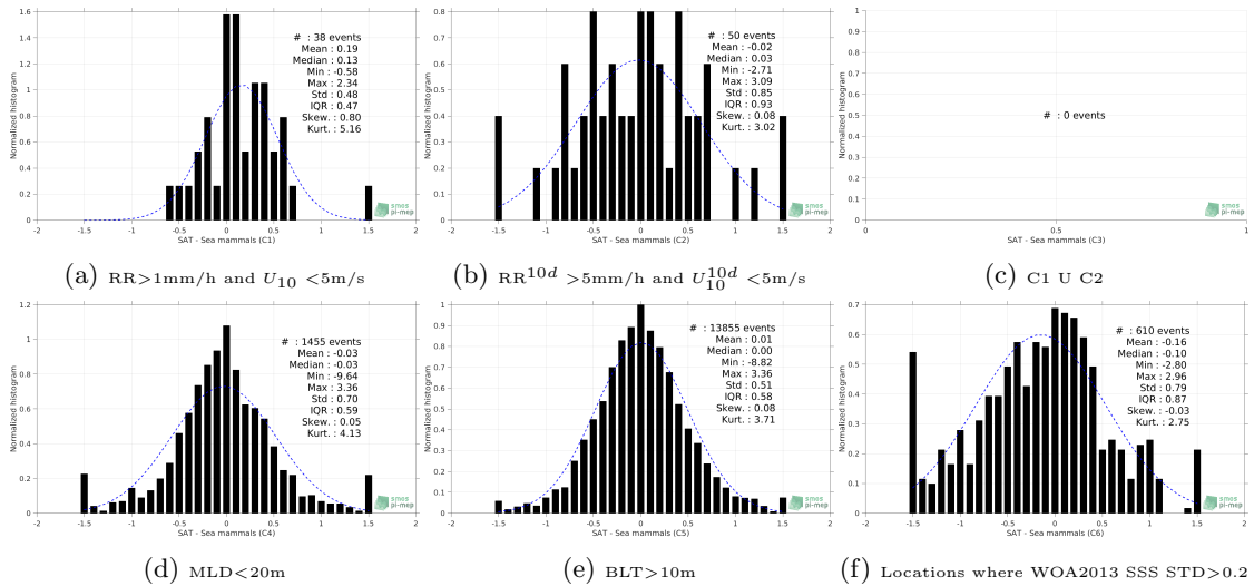
Figure 13: Normalized histogram of \Delta\text{SSS} (SMOS-L4-CATDS-CECOS-IFREMER-V2-WEEKLY-0.5DEG - Sea mammals) for 6 different subdatasets corresponding to: RR > 1\text{mm/h} and U_{10} < 5\text{m/s} (a), RR^{10d} > 5\text{mm/h} and U_{10}^{10d} < 5\text{m/s} (b), C1 U C2 (c), MLD < 20\text{m} (d), BLT > 10\text{m} (e), Locations where WOA2013 SSS STD > 0.2 (f).
