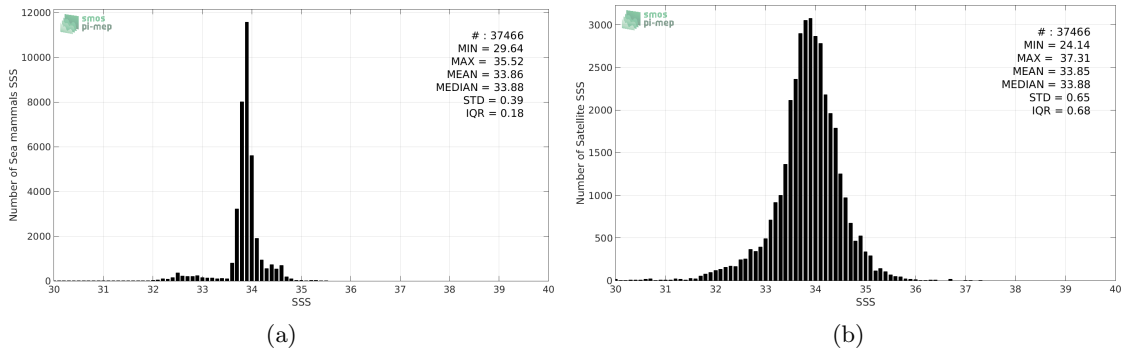
Figure 2: Histograms of SSS from Sea mammals (a) and SMOS-L4-CATDS-CECOS-IFREMER-V2-WEEKLY-0.5DEG (b) considering all match-up pairs per bins of 0.1 over the SMOS coastal zone ( \geq 800\text{km} ) 60N-60S Pi-MEP region and for the full satellite product period.
