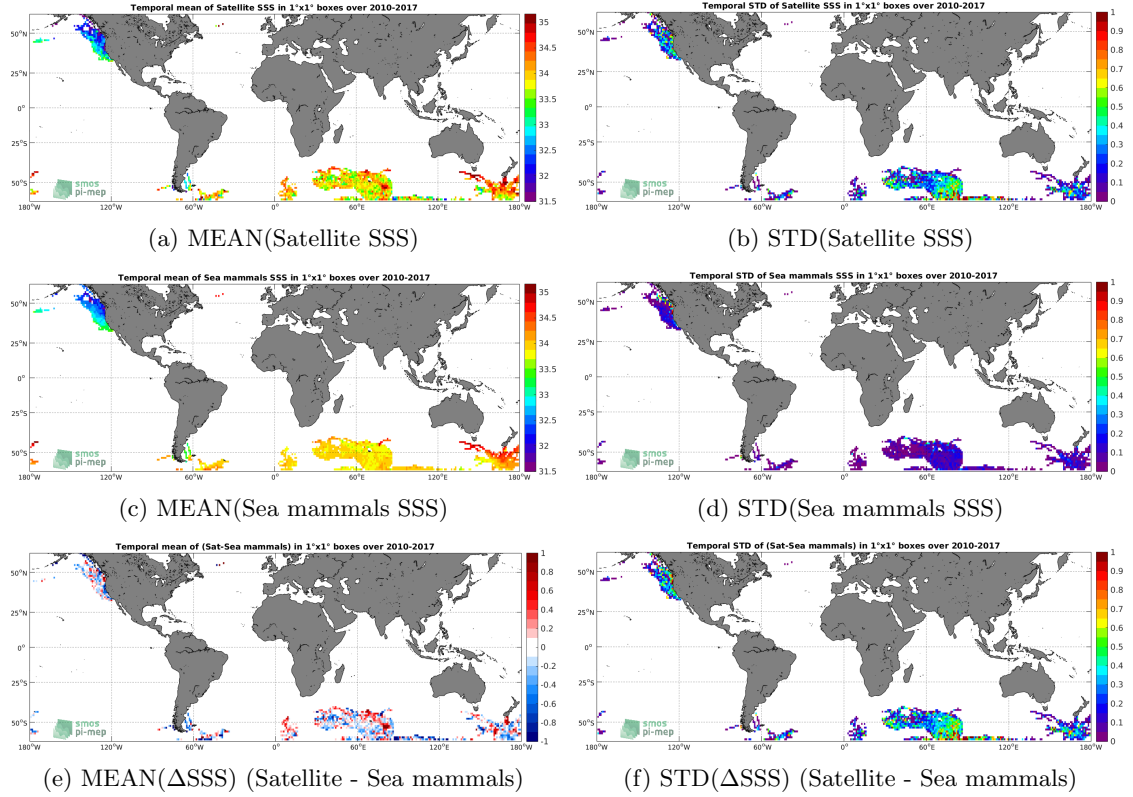
Figure 6: Temporal mean (left) and STD (right) of SSS from SMOS-L4-CATDS-CECOS-IFREMER-V2-WEEKLY-0.5DEG (top), Sea mammals (middle), and of \Delta SSS (Satellite - Sea mammals). Only match-up pairs are used to generate these maps.
