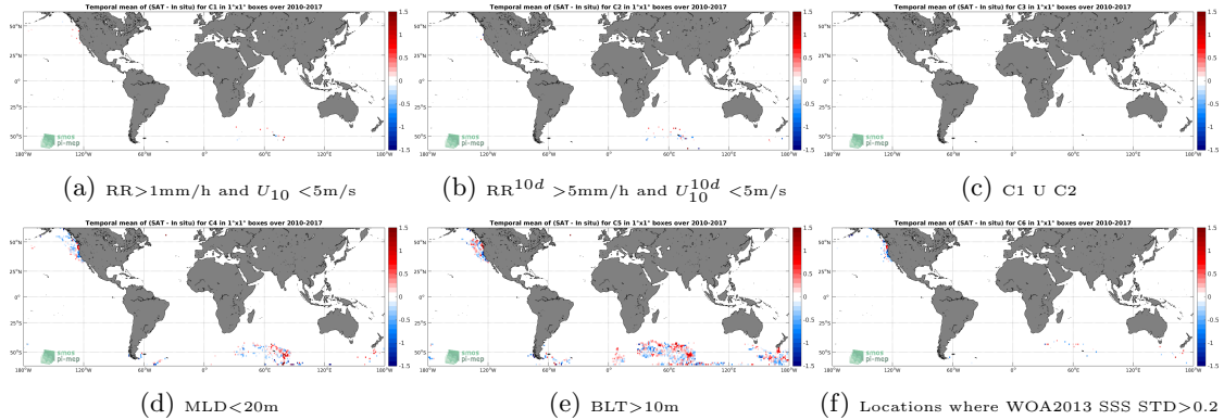
Figure 12: Temporal mean gridded over spatial boxes of size 1^\circ \times 1^\circ of \Delta\text{SSS} (SMOS-L4-CATDS-CECOS-IFREMER-V2-WEEKLY-0.5DEG - Sea mammals) for 6 different subdatasets corresponding to: RR > 1\text{mm/h} and U_{10} < 5\text{m/s} (a), RR^{10d} > 5\text{mm/h} and U_{10}^{10d} < 5\text{m/s} (b), C1 U C2 (c), MLD < 20\text{m} (d), BLT > 10\text{m} (e), Locations where WOA2013 SSS STD > 0.2 (f).
