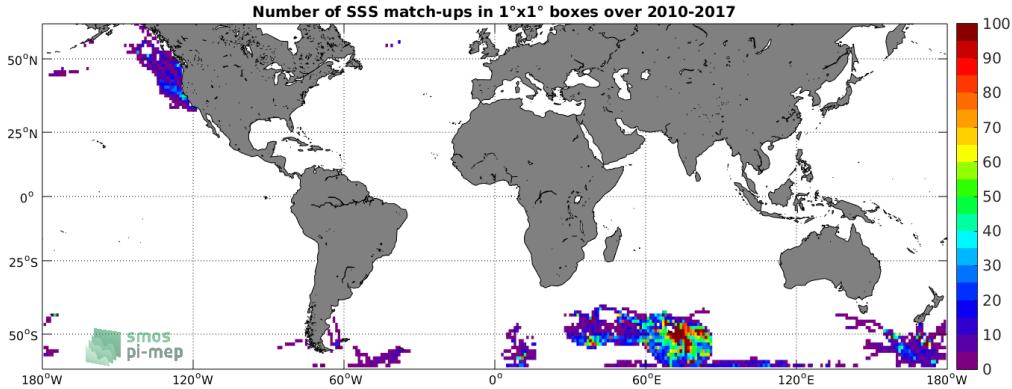
Figure 4: Number of SSS match-ups between Sea mammals SSS and the SMOS-L4-CATDS-CECOS-IFREMER-V2-WEEKLY-0.5DEG SSS product for the SMOS coastal zone ( \leq 800\text{km} ) 60N-60S Pi-MEP region over 1^\circ \times 1^\circ boxes and for the full satellite product period.
