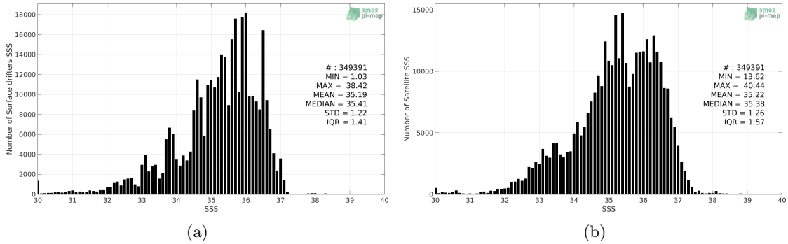
Figure 2: Histograms of SSS from Surface drifters (a) and SMOS-L4-CATDS-CECOS-IFREMER-V2-WEEKLY-0.5DEG (b) considering all match-up pairs per bins of 0.1 over the SMOS coastal zone ( \geq 800\text{km} ) 60N-60S Pi-MEP region and for the full satellite product period.
