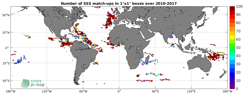
Figure 3: Number of SSS match-ups between Surface drifters SSS and the SMOS-L4-CATDS-CECOS-IFREMER-V2-WEEKLY-0.5DEG SSS product for the SMOS coastal zone ( \geq 800\text{km} ) 60N-60S Pi-MEP region over 1^\circ \times 1^\circ boxes and for the full satellite product period.
