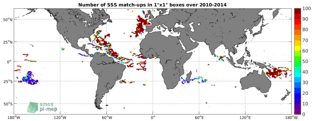
Figure 3: Number of SSS match-ups between Surface drifters SSS and the SMOS-L4-CATDS-CECOS-IFREMER-V2-WEEKLY-0.5DEG SSS product for the SMOS coastal zone ( \approx 800\text{km} ) 60N-60S Pi-MEP region over 1^\circ \times 1^\circ boxes and for the full satellite product period.
