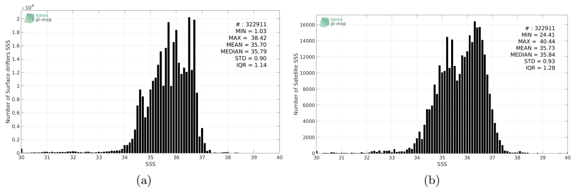
Figure 2: Histograms of SSS from Surface drifters (a) and SMOS-L4-CATDS-CECOS-IFREMER-V2-WEEKLY-0.5DEG (b) considering all match-up pairs per bins of 0.1 over the SMOS coastal zone ( \approx 800\text{km} ) 60N-60S Pi-MEP region and for the full satellite product period.
