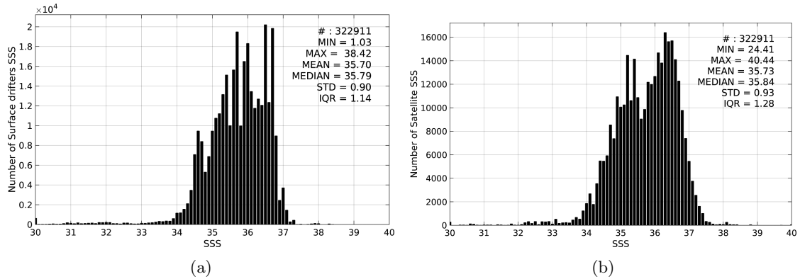
Figure 2: Histograms of SSS from Surface drifters (a) and SMOS-L4-CATDS-CECOS-IFREMER-V2-WEEKLY-0.5DEG (b) considering all match-up pairs per bins of 0.1 over the SMOS coastal zone ( \pm 800\text{km} ) 60N-60S Pi-MEP region and for the full satellite product period.
