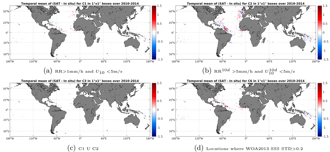
Figure 11: Temporal mean gridded over spatial boxes of size 1^\circ \times 1^\circ of \Delta SSS (SMOS-L4-CATDS-CECOS-IFREMER-V2-WEEKLY-0.5DEG - Surface drifters) for 4 different subdatasets corresponding to: RR > 1\text{mm/h} and U_{10} < 5\text{m/s} (a), RR^{10d} > 5\text{mm/h} and U_{10}^{10d} < 5\text{m/s} (b), C1 U C2 (c), Locations where WOA2013 SSS STD > 0.2 (d).
