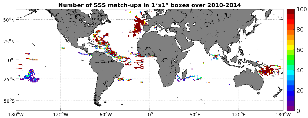
Figure 3: Number of SSS match-ups between Surface drifters SSS and the SMOS-L4-CATDS-CECOS-IFREMER-V2-WEEKLY-0.5DEG SSS product for the SMOS coastal zone ( \pm 800\text{km} ) 60N-60S Pi-MEP region over 1^\circ \times 1^\circ boxes and for the full satellite product period.
