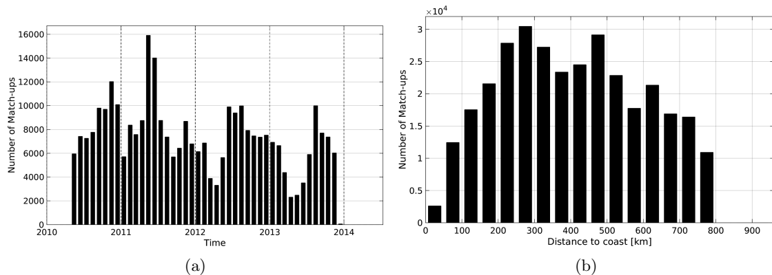
Figure 1: Number of match-ups between Surface drifters and SMOS-L4-CATDS-CECOS-IFREMER-V2-WEEKLY-0.5DEG SSS as a function of time (a) and as function of the distance to coast (b) over the SMOS coastal zone ( \pm 800 km) 60N-60S Pi-MEP region and for the full satellite product period.
