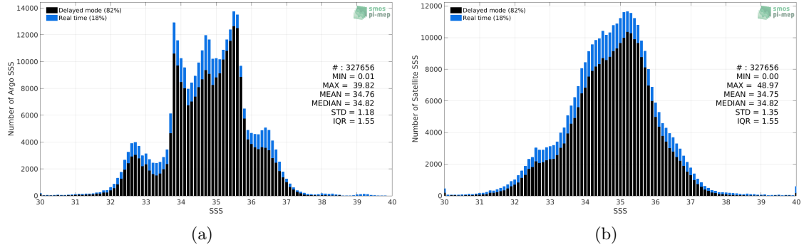
Figure 2: Histograms of SSS from Argo (a) and SMOS L4 v2 Weekly (CATDS-CECOS-IFREMER) (b) considering all match-up pairs per bins of 0.1 over the SMOS coastal zone (<800km) 60N-60S Pi-MEP region and for the full satellite product period.
