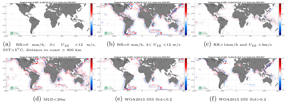
Figure 12: Temporal mean gridded over spatial boxes of size 1^\circ \times 1^\circ of \Delta SSS (SMOS L4 v2 Weekly (CATDS-CECOS-IFREMER) - Argo) for 6 different subdatasets corresponding to:RR=0 mm/h, 3 < U_{10} < 12 m/s, SST > 5^\circ\text{C} , distance to coast > 800 km (a), RR=0 mm/h, 3 < U_{10} < 12 m/s (b), RR > 1 mm/h and U_{10} < 4 m/s (c),MLD < 20 m (d),WOA2013 SSS Std < 0.2 (e),WOA2013 SSS Std > 0.2 (f).
