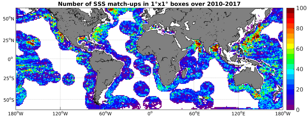
Figure 4: Number of SSS match-ups between Argo SSS and the SMOS-L4-CATDS-CECOS-IFREMER-V2-WEEKLY-0.5DEG SSS product for the SMOS coastal zone ( \approx 800\text{km} ) 60N-60S Pi-MEP region over 1°x1° boxes and for the full satellite product period.
