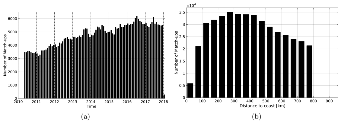
Figure 1: Number of match-ups between Argo and SMOS-L4-CATDS-CECOS-IFREMER-V2-WEEKLY-0.5DEG SSS as a function of time (a) and as function of the distance to coast (b) over the SMOS coastal zone ( \pm 800 km) 60N-60S Pi-MEP region and for the full satellite product period.
