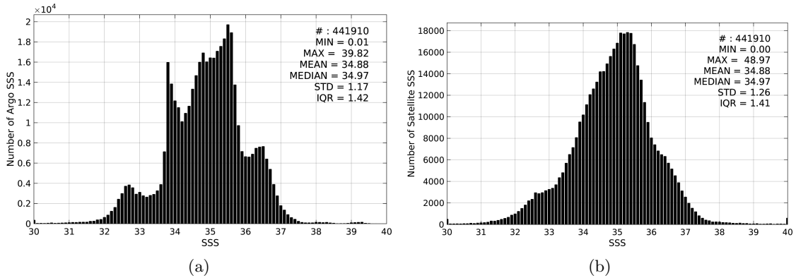
Figure 2: Histograms of SSS from Argo (a) and SMOS-L4-CATDS-CECOS-IFREMER-V2-WEEKLY-0.5DEG (b) considering all match-up pairs per bins of 0.1 over the SMOS coastal zone ( \approx 800\text{km} ) 60N-60S Pi-MEP region and for the full satellite product period.
