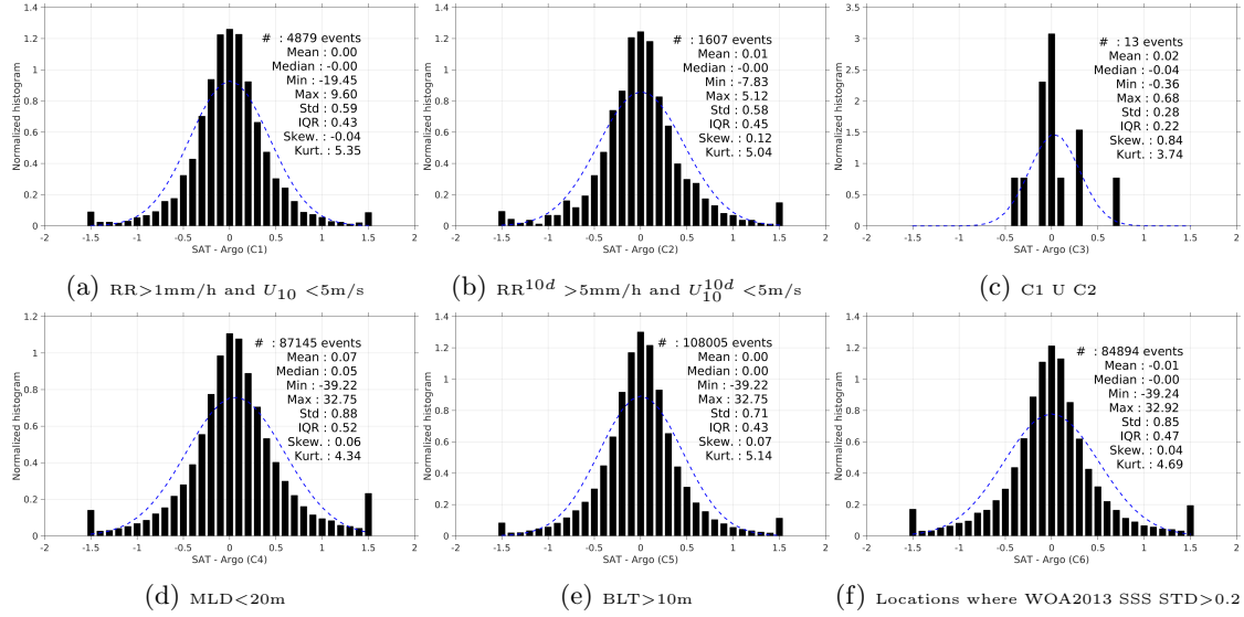
Figure 13: Normalized histogram of \Delta SSS (SMOS-L4-CATDS-CECOS-IFREMER-V2-WEEKLY-0.5DEG - Argo) for 6 different subdatasets corresponding to: RR>1mm/h and U_{10} <5m/s (a), RR 10d >5mm/h and U_{10}^{10d} <5m/s (b), C1 U C2 (c),MLD<20m (d),BLT>10m (e),Locations where WOA2013 SSS STD>0.2 (f).
