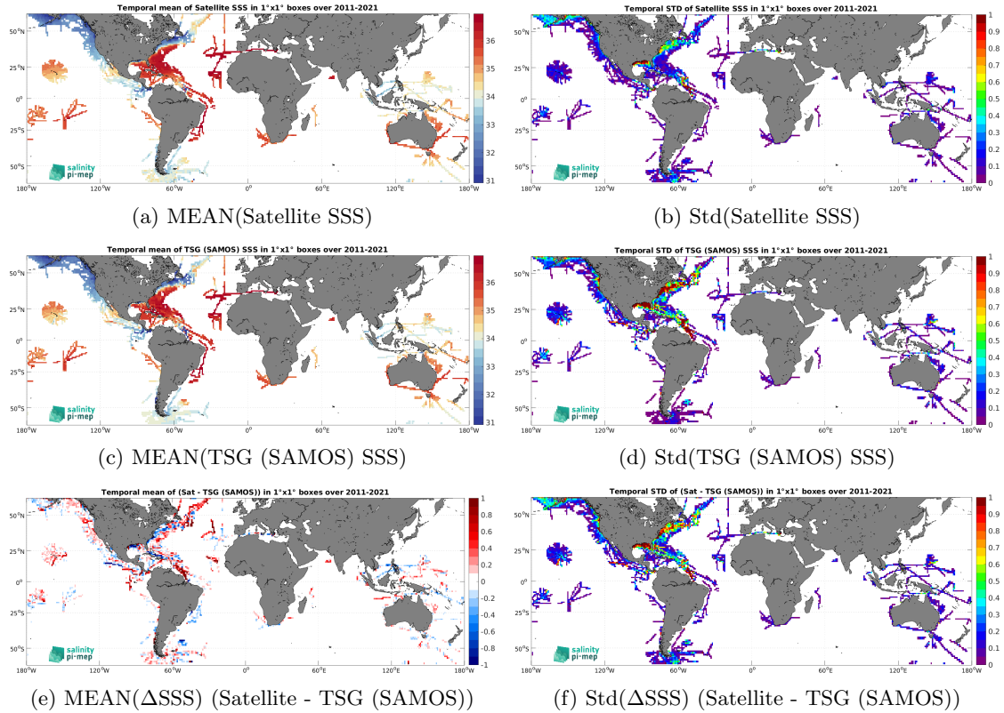
Figure 7: Temporal mean (left) and Std (right) of SSS from SMOS SSS L4 v2 - Daily (BEC) (top), TSG (SAMOS) (middle), and of \Delta SSS (Satellite - TSG (SAMOS)). Only match-up pairs are used to generate these maps.
