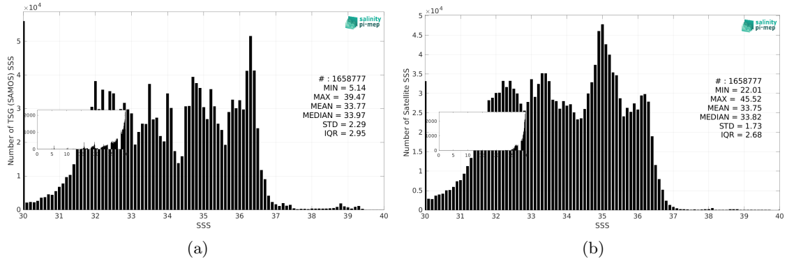
Figure 3: Histograms of SSS from TSG (SAMOS) (a) and SMOS SSS L4 v2 - Daily (BEC) (b) considering all match-up pairs per bins of 0.1 over the SMOS coastal zone (<800km) 60N-60S Pi-MEP region and for the full satellite product period.
