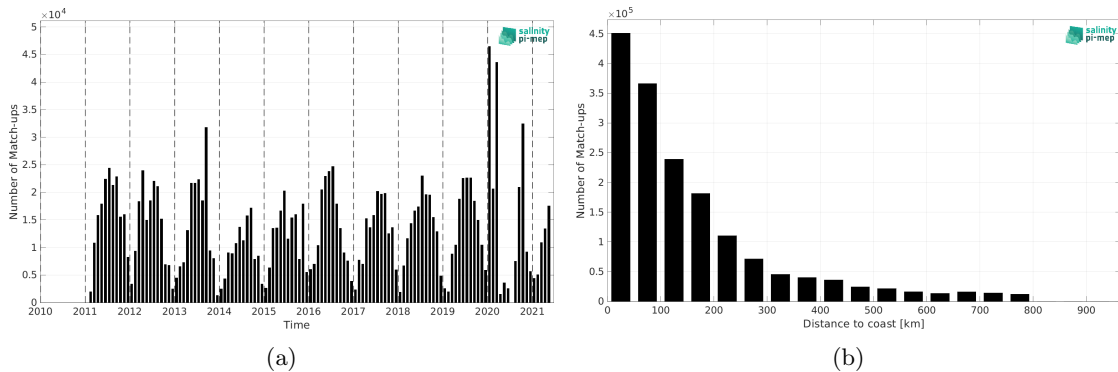
Figure 2: Number of match-ups between TSG (SAMOS) and SMOS SSS L4 v2 - Daily (BEC) SSS as a function of time (a) and as function of the distance to coast (b) over the SMOS coastal zone (<800km) 60N-60S Pi-MEP region and for the full satellite product period.
