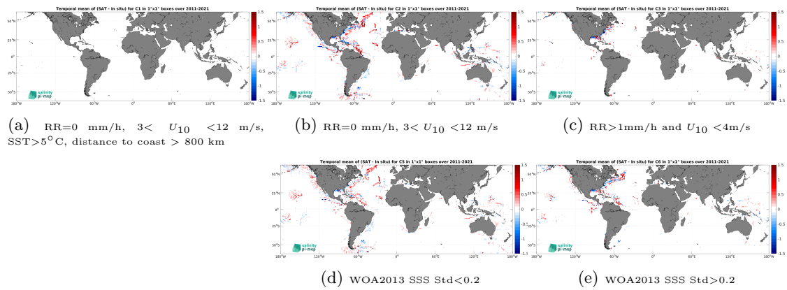
Figure 14: Temporal mean gridded over spatial boxes of size 1^\circ \times 1^\circ of \Delta\text{SSS} (SMOS SSS L4 v2 - Daily (BEC) - TSG (SAMOS)) for 5 different subdatasets corresponding to:RR=0 mm/h, 3 < U_{10} < 12 m/s, SST >5^\circ\text{C} , distance to coast > 800 km (a), RR=0 mm/h, 3 < U_{10} < 12 m/s (b), RR >1 mm/h and U_{10} < 4 m/s (c), WOA2013 SSS Std <0.2 (d), WOA2013 SSS Std >0.2 (e).
