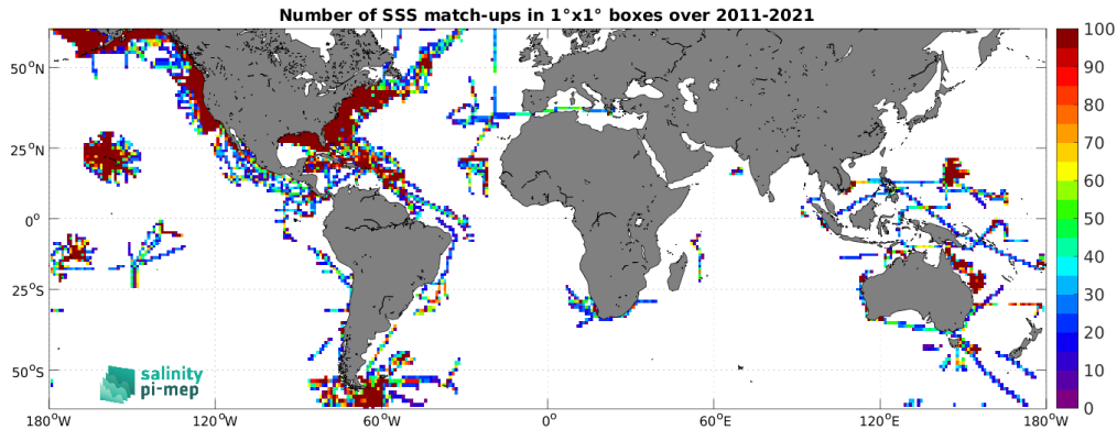
Figure 5: Number of SSS match-ups between TSG (SAMOS) SSS and the SMOS SSS L4 v2 - Daily (BEC) SSS product for the SMOS coastal zone (<800km) 60N-60S Pi-MEP region over 1^\circ \times 1^\circ boxes and for the full satellite product period.
