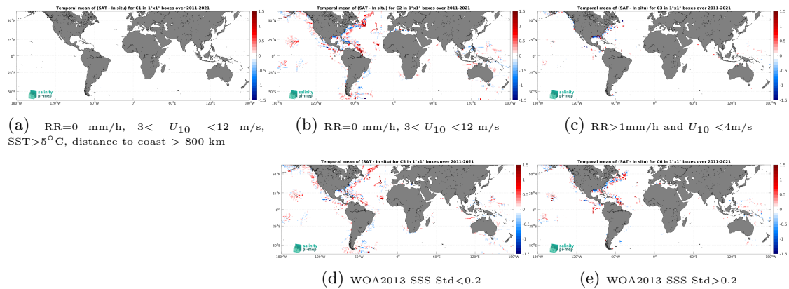
Figure 12: Temporal mean gridded over spatial boxes of size 1^\circ \times 1^\circ of \Delta SSS (SMOS SSS L4 v2 - Daily (BEC) - TSG (SAMOS)) for 5 different subdatasets corresponding to:RR=0 mm/h, 3 < U_{10} < 12 m/s, SST >5^\circ\text{C} , distance to coast > 800 km (a), RR=0 mm/h, 3 < U_{10} < 12 m/s (b), RR >1 mm/h and U_{10} < 4 m/s (c), WOA2013 SSS Std <0.2 (d), WOA2013 SSS Std >0.2 (e).
