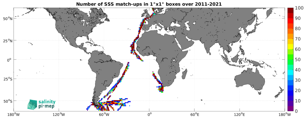
Figure 5: Number of SSS match-ups between TSG (Polarstern) SSS and the SMOS SSS L4 v2 - Daily (BEC) SSS product for the SMOS coastal zone (<800km) 60N-60S Pi-MEP region over 1^\circ \times 1^\circ boxes and for the full satellite product period.
