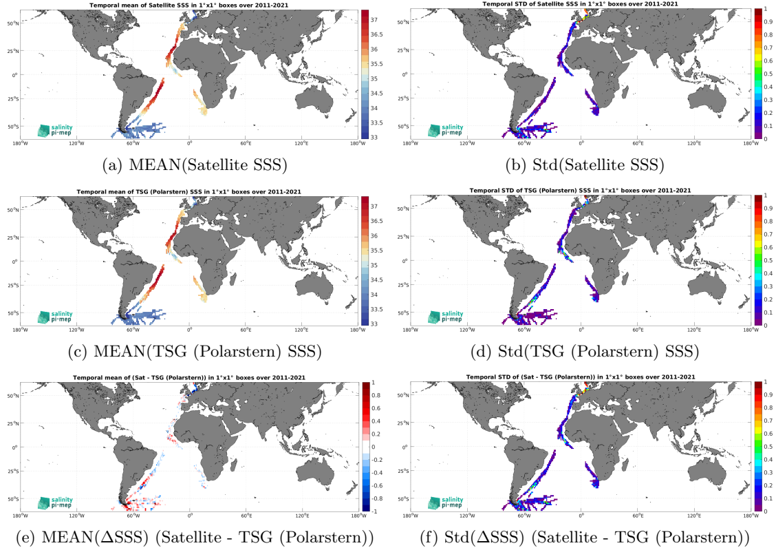
Figure 7: Temporal mean (left) and Std (right) of SSS from SMOS SSS L4 v2 - Daily (BEC) (top), TSG (Polarstern) (middle), and of \Delta SSS (Satellite - TSG (Polarstern)). Only match-up pairs are used to generate these maps.
