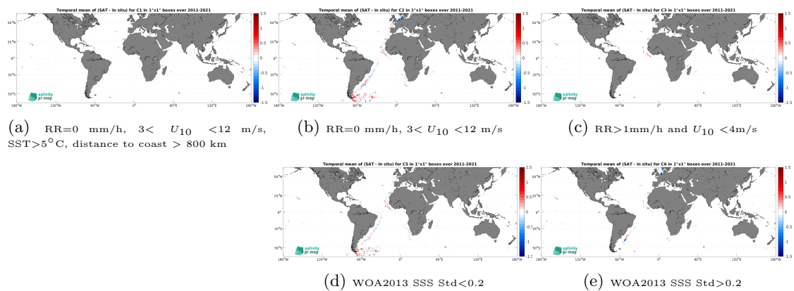
Figure 14: Temporal mean gridded over spatial boxes of size 1^\circ \times 1^\circ of \Delta\text{SSS} (SMOS SSS L4 v2 - Daily (BEC) - TSG (Polarstern)) for 5 different subdatasets corresponding to:RR=0 mm/h, 3 < U_{10} < 12 m/s, SST>5°C, distance to coast > 800 km (a), RR=0 mm/h, 3 < U_{10} < 12 m/s (b), RR>1mm/h and U_{10} < 4 m/s (c), WOA2013 SSS Std<0.2 (d), WOA2013 SSS Std>0.2 (e).
