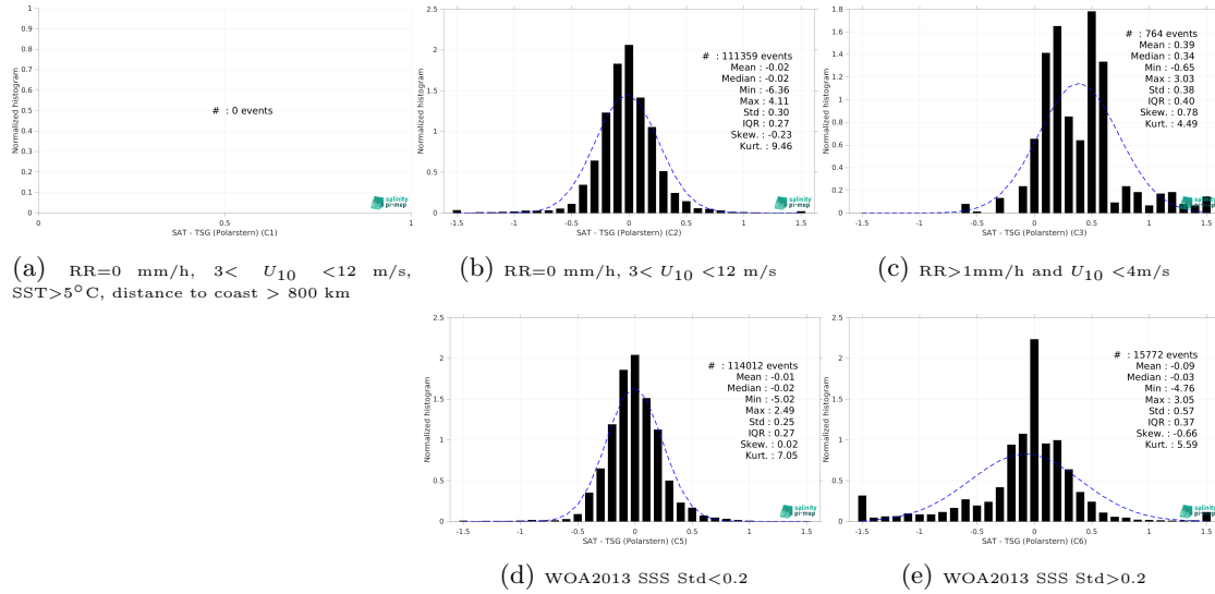
Figure 15: Normalized histogram of \Delta SSS (SMOS SSS L4 v2 - Daily (BEC) - TSG (Polarstern)) for 5 different subdatasets corresponding to: RR=0 mm/h, 3 < U_{10} < 12 m/s, SST > 5°C, distance to coast > 800 km (a), RR=0 mm/h, 3 < U_{10} < 12 m/s (b), RR > 1mm/h and U_{10} < 4 m/s (c), WOA2013 SSS Std < 0.2 (d), WOA2013 SSS Std > 0.2 (e).
