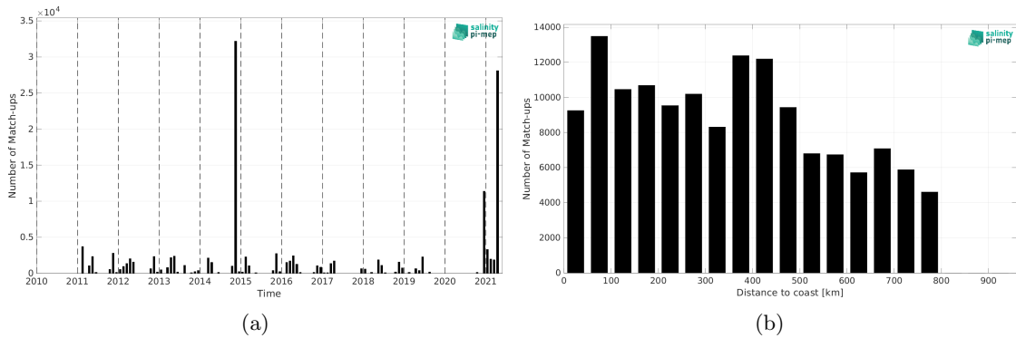
Figure 2: Number of match-ups between TSG (Polarstern) and SMOS SSS L4 v2 - Daily (BEC) SSS as a function of time (a) and as function of the distance to coast (b) over the SMOS coastal zone (<800km) 60N-60S Pi-MEP region and for the full satellite product period.
