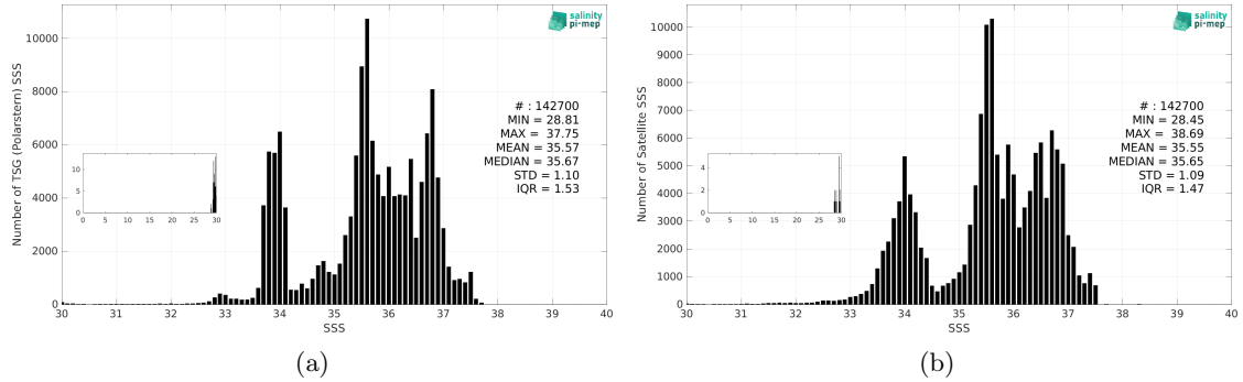
Figure 3: Histograms of SSS from TSG (Polarstern) (a) and SMOS SSS L4 v2 - Daily (BEC) (b) considering all match-up pairs per bins of 0.1 over the SMOS coastal zone (<800km) 60N-60S Pi-MEP region and for the full satellite product period.
