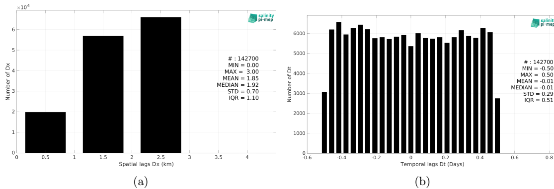
Figure 6: Histograms of the spatial (a) and temporal (b) lags between the location/time of the TSG (Polarstern) measurement and the date of the corresponding SMOS SSS L4 v2 - Daily (BEC) SSS pixel.
