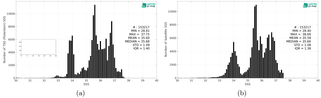
Figure 2: Histograms of SSS from TSG (Polarstern) (a) and SMOS SSS L4 v2 - Daily (BEC) (b) considering all match-up pairs per bins of 0.1 over the SMOS coastal zone (<800km) 60N-60S Pi-MEP region and for the full satellite product period.
