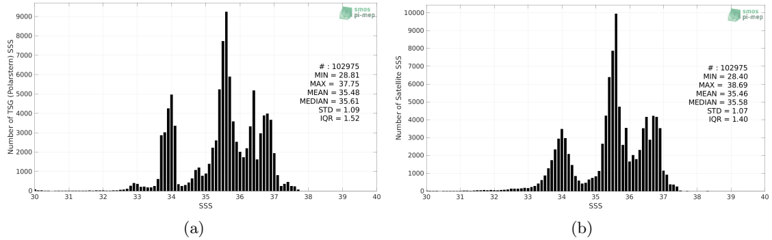
Figure 2: Histograms of SSS from TSG (Polarstern) (a) and SMOS SSS L4 v2 - Daily (BEC) (b) considering all match-up pairs per bins of 0.1 over the SMOS coastal zone (<800km) 60N-60S Pi-MEP region and for the full satellite product period.
