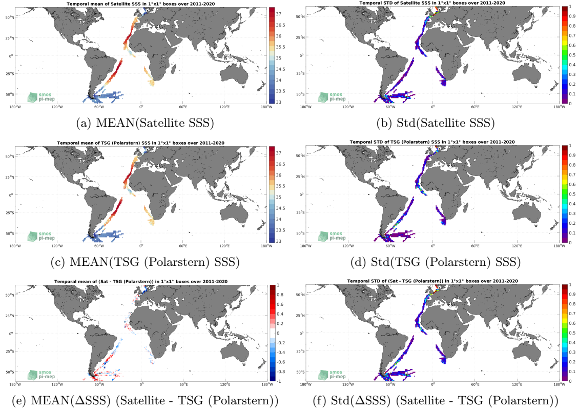
Figure 6: Temporal mean (left) and Std (right) of SSS from SMOS SSS L4 v2 - Daily (BEC) (top), TSG (Polarstern) (middle), and of \Delta SSS (Satellite - TSG (Polarstern)). Only match-up pairs are used to generate these maps.
