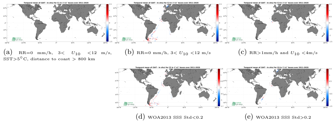
Figure 12: Temporal mean gridded over spatial boxes of size 1^\circ \times 1^\circ of \Delta SSS (SMOS SSS L4 v2 - Daily (BEC) - TSG (Polarstern)) for 5 different subdatasets corresponding to:RR=0 mm/h, 3 < U_{10} < 12 m/s, SST > 5^\circ\text{C} , distance to coast > 800 km (a), RR=0 mm/h, 3 < U_{10} < 12 m/s (b), RR > 1 mm/h and U_{10} < 4 m/s (c), WOA2013 SSS Std < 0.2 (d), WOA2013 SSS Std > 0.2 (e).
