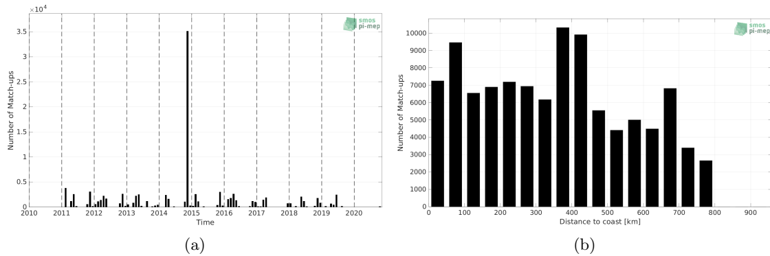
Figure 1: Number of match-ups between TSG (Polarstern) and SMOS SSS L4 v2 - Daily (BEC) SSS as a function of time (a) and as function of the distance to coast (b) over the SMOS coastal zone (<800km) 60N-60S Pi-MEP region and for the full satellite product period.
