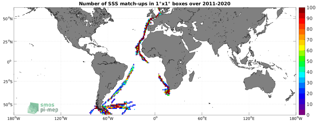
Figure 4: Number of SSS match-ups between TSG (Polarstern) SSS and the SMOS SSS L4 v2 - Daily (BEC) SSS product for the SMOS coastal zone (<800km) 60N-60S Pi-MEP region over 1^\circ \times 1^\circ boxes and for the full satellite product period.
