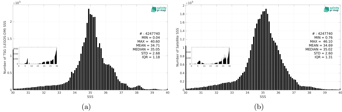
Figure 3: Histograms of SSS from TSG (LEGOS-DM) (a) and SMOS SSS L4 v2 - Daily (BEC) (b) considering all match-up pairs per bins of 0.1 over the SMOS coastal zone (<800km) 60N-60S Pi-MEP region and for the full satellite product period.
