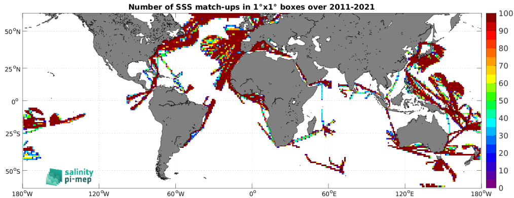
Figure 5: Number of SSS match-ups between TSG (LEGOS-DM) SSS and the SMOS SSS L4 v2 - Daily (BEC) SSS product for the SMOS coastal zone (<800km) 60N-60S Pi-MEP region over 1^\circ \times 1^\circ boxes and for the full satellite product period.
