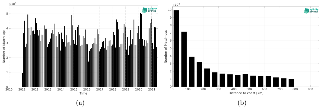
Figure 2: Number of match-ups between TSG (LEGOS-DM) and SMOS SSS L4 v2 - Daily (BEC) SSS as a function of time (a) and as function of the distance to coast (b) over the SMOS coastal zone (<800km) 60N-60S Pi-MEP region and for the full satellite product period.
