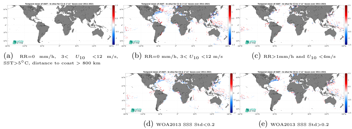
Figure 14: Temporal mean gridded over spatial boxes of size 1^\circ \times 1^\circ of \Delta\text{SSS} (SMOS SSS L4 v2 - Daily (BEC) - TSG (LEGOS-DM)) for 5 different subdatasets corresponding to: RR=0 mm/h, 3 < U_{10} < 12 m/s, SST > 5°C, distance to coast > 800 km (a), RR=0 mm/h, 3 < U_{10} < 12 m/s (b), RR > 1mm/h and U_{10} < 4 m/s (c), WOA2013 SSS Std < 0.2 (d), WOA2013 SSS Std > 0.2 (e).
