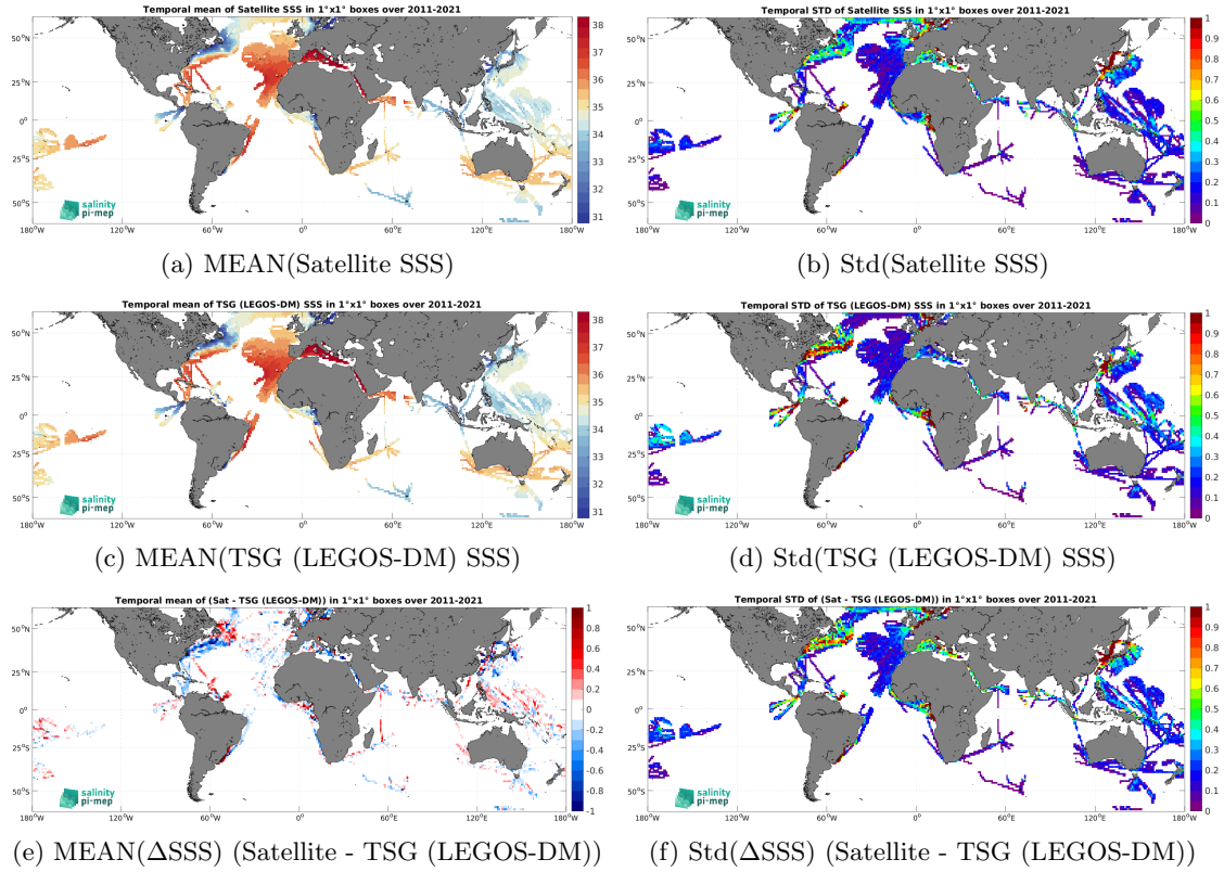
Figure 7: Temporal mean (left) and Std (right) of SSS from SMOS SSS L4 v2 - Daily (BEC) (top), TSG (LEGOS-DM) (middle), and of \Delta SSS (Satellite - TSG (LEGOS-DM)). Only match-up pairs are used to generate these maps.
