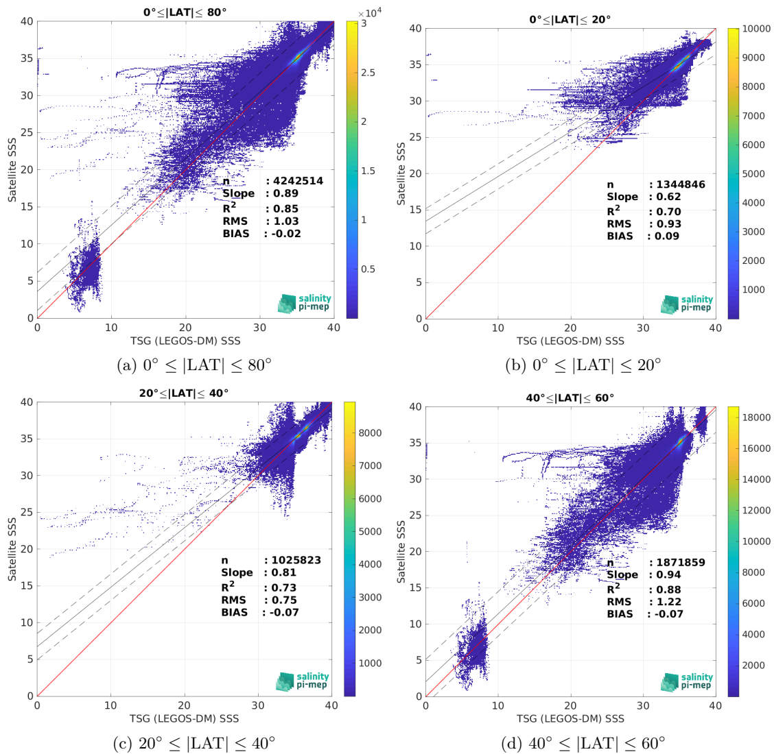
Figure 10: Contour maps of the concentration of SMOS SSS L4 v2 - Daily (BEC) SSS (y-axis) versus TSG (LEGOS-DM) SSS (x-axis) at match-up pairs for different latitude bands. For each plot, the red line shows x=y . The black thin and dashed lines indicate a linear fit through the data cloud and the \pm 95\% confidence levels, respectively. The number match-up pairs n , the slope and R^2 coefficient of the linear fit, the root mean square (RMS) and the mean bias between satellite and in situ data are indicated for each latitude band in each plots.
